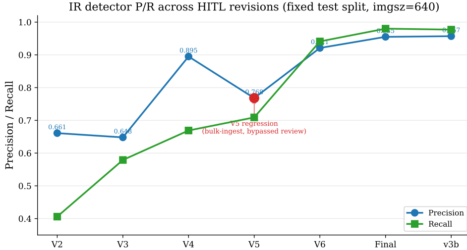
Figure 5.2: IR detector P/R trajectory across the five numbered revisions (V2–V6) plus the Final retrain and production v3b , on the fixed IR_dset_final test split. The V5 regression (precision 0.895 \rightarrow 0.768) is recovered by V6 and the production v3b .
