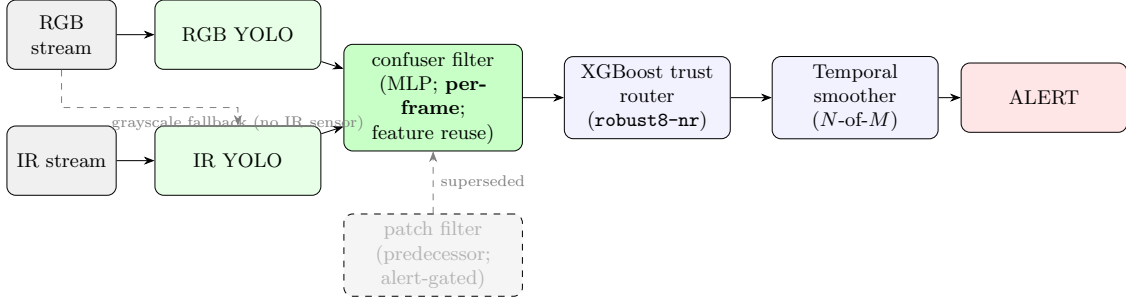
Figure 3.1: Multi-stage drone detection pipeline in the production composition: detectors, then the confuser filter, then the trust classifier. The order itself was ablated (Section 5.1): filter-first ships because it edges classifier-first on Svanström ( F1 = 0.946 vs 0.931 ), and the two are within about a point on the paired benchmarks. The production confuser filter is the distilled mlp_v5_v4 (RGB) with its paired thermal-native IR head, which runs per frame because it reuses the detectors’ already-computed internal features rather than re-processing crops (Section 3.9). It supersedes the MobileNetV3 patch filter (greyed), which was expensive enough that it had to be alert-gated : consulted only when the temporal smoother was about to fire (Section F.2).
