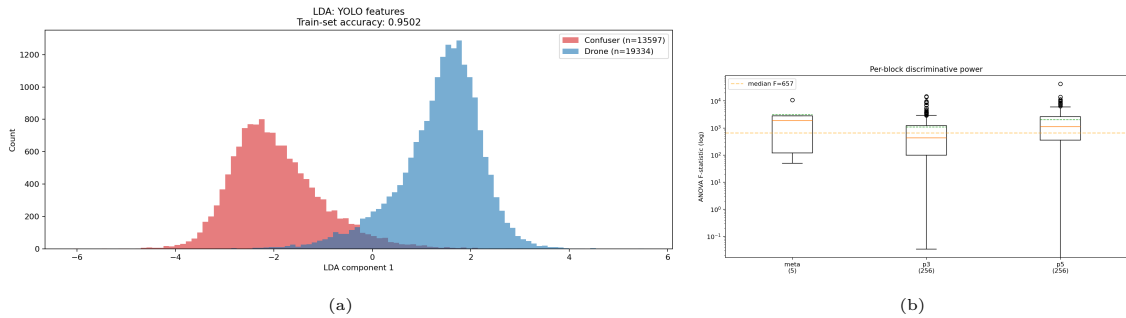
Figure 5.4: Model MRI of the FT4 detector’s fused p3+p5 features on the shipped 32,931-detection corpus. (a) The linear-discriminant projection separates drone (blue) from confuser (red) into two cleanly-resolved peaks at \approx 95\% single-threshold accuracy. (b) Per-block ANOVA F -statistic: p5 is the dominant discriminative layer (max F = 42,346 , median 657), ahead of p3 and the detection metadata; the confidence scalar ranks only 6th.
