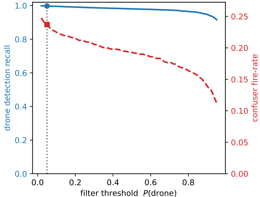
IR-thermal aligned (shipped t = 0.05 )
