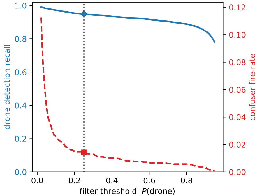
RGB mlp_v5_v4 (shipped t = 0.25 )
