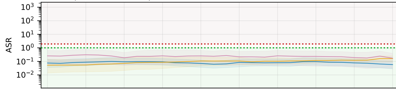
Stratospheric ozone depletion (SOD)
