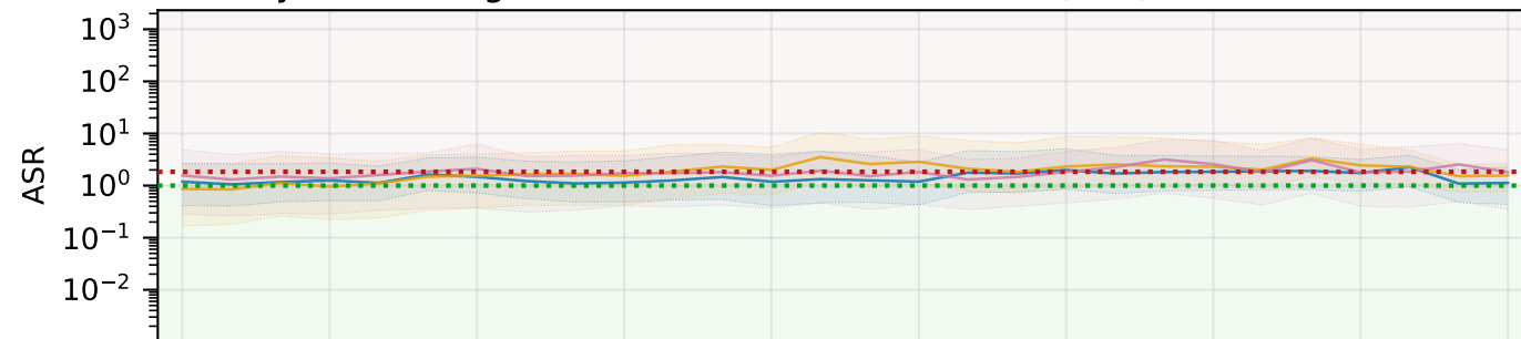
Land-system change: Global area of forested land (LSC)
