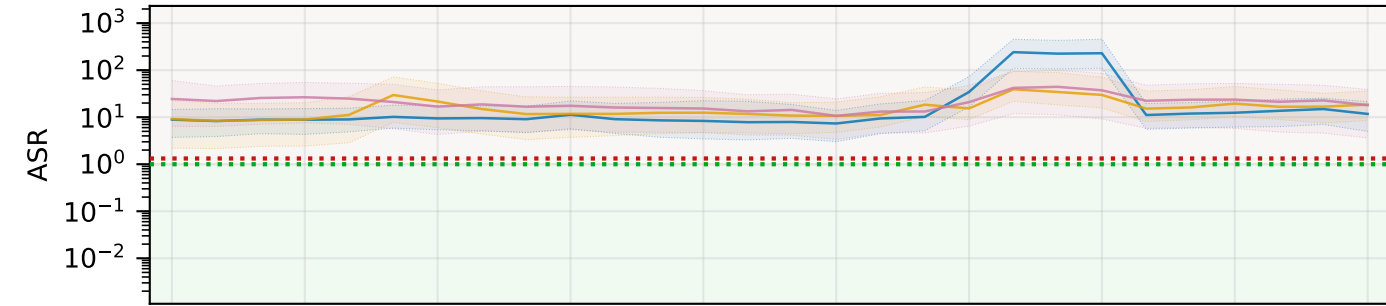
Biogeochemical flows: Nitrogen (N)
