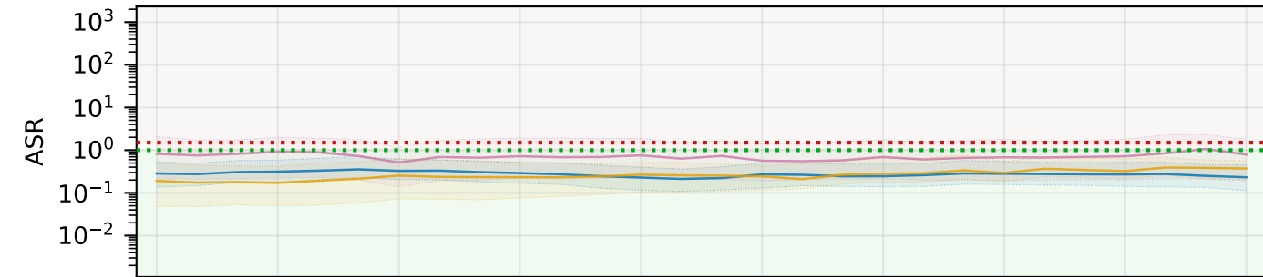
Freshwater use: Blue water (FWU)
