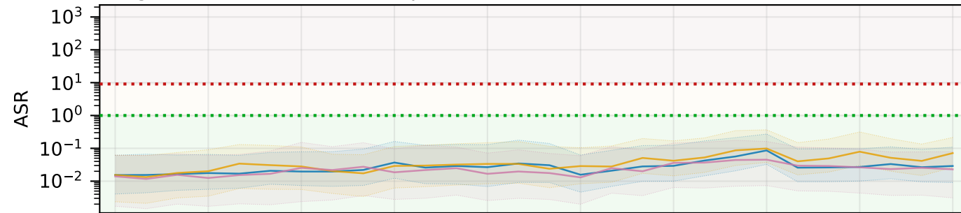
Biogeochemical flows: Phosphorus (P GLO)
