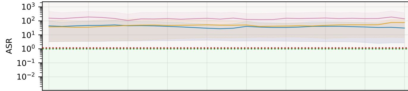
Ocean acidification (OA)
