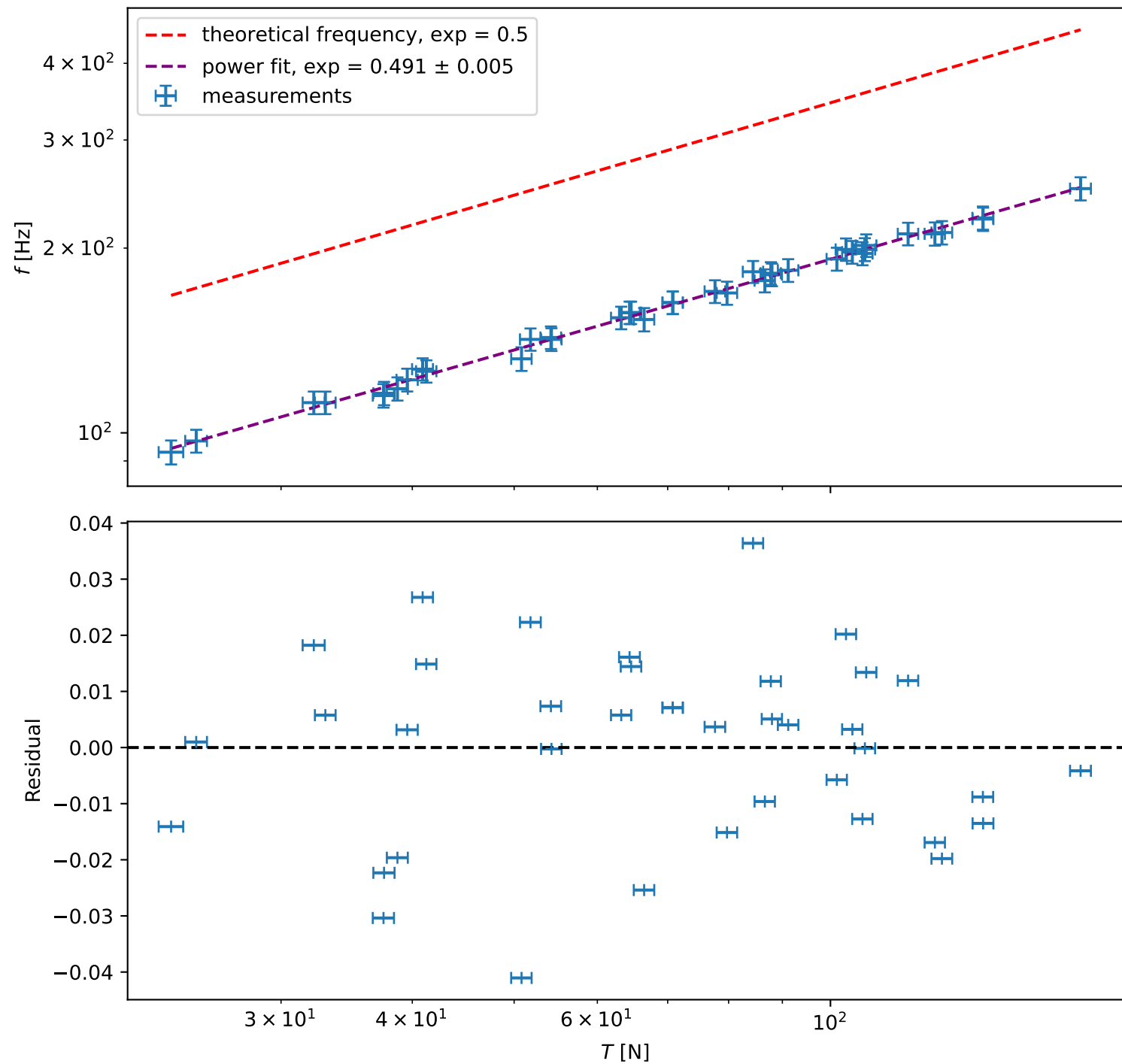
Frequency Dependence on Tension
