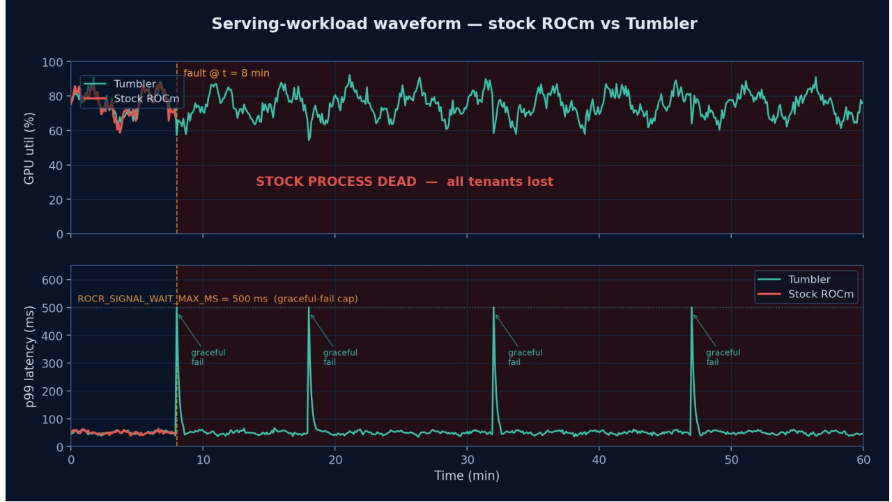
Figure 3. Serving-workload waveform on the same AI inference reproducer. Both runs start at the same baseline ( \approx 75\% GPU util, \approx 50 ms p99 latency). At t = 8 min a transient fault hits. Stock ROCm aborts: util and latency go away (red band). Tumbler shows a brief bounded latency spike at the ROCR_SIGNAL_WAIT_MAX_MS = 500 ms cap, then the workload recovers; subsequent hiccups behave the same way.
