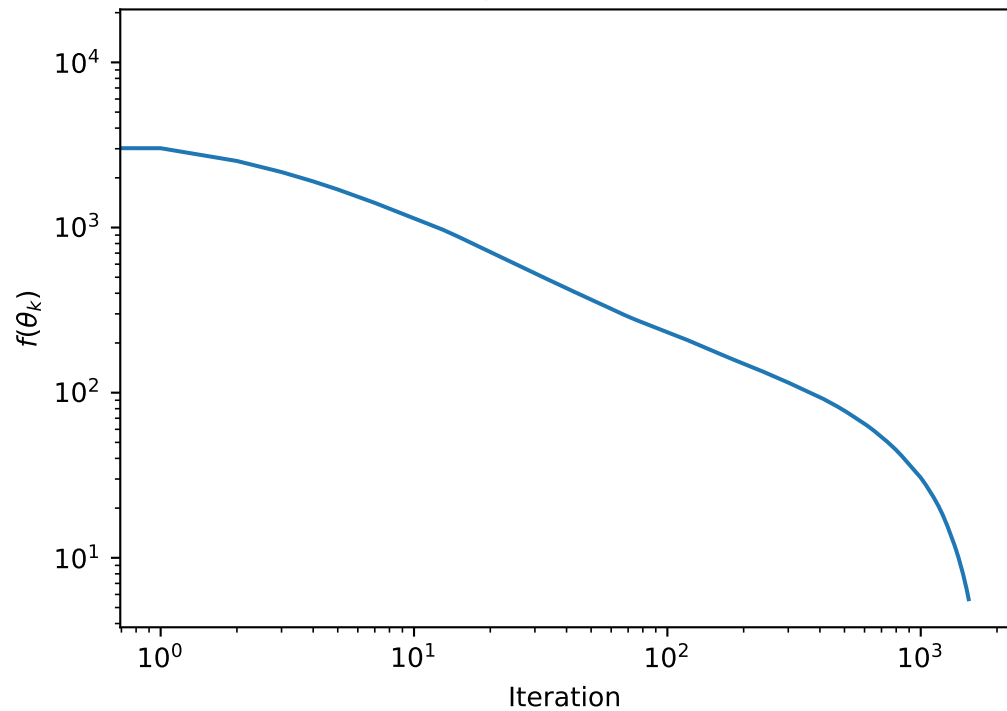
Objective value
