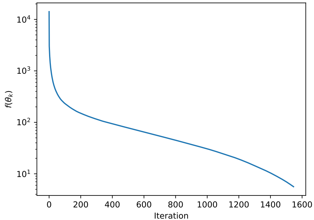
Objective value
