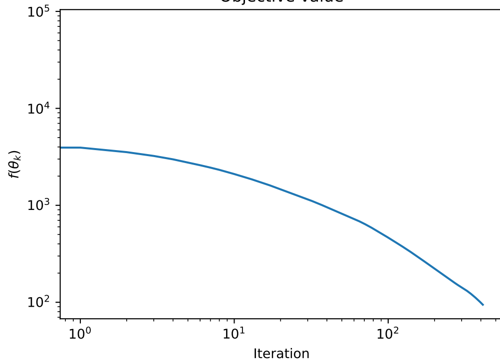
Objective value
