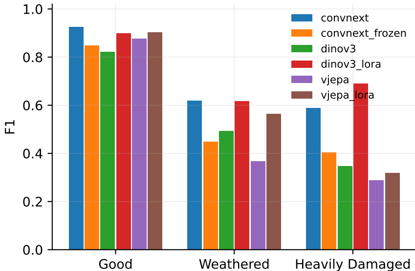
MTSD attributes - condition head per-class F1 (weakest head)
