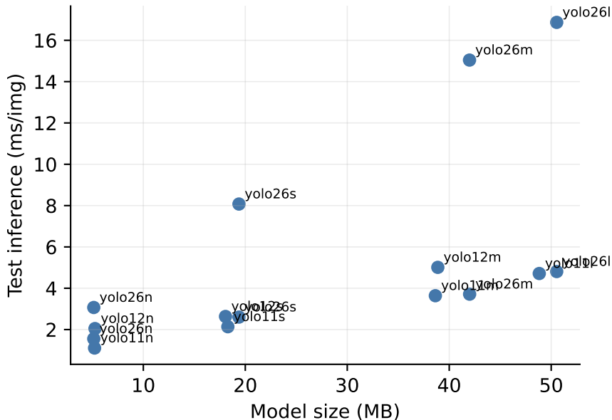
MDWD detection - latency vs model size (val-time measurement)
