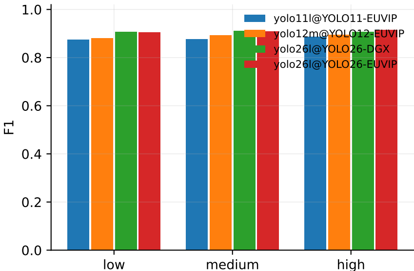
MDWD detection - F1 by image brightness (test)
