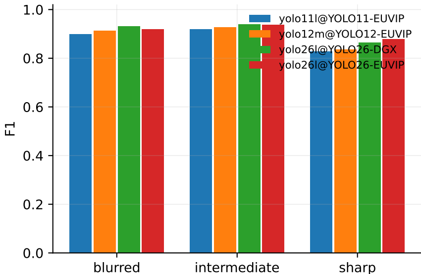
MDWD detection - F1 by image sharpness (test)
