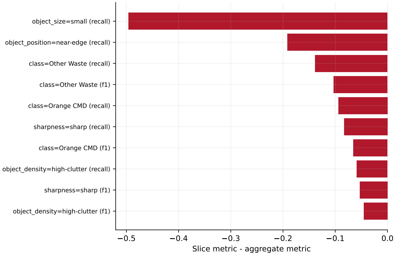
MDWD detection - largest slice deviations (test, worst model per slice)
