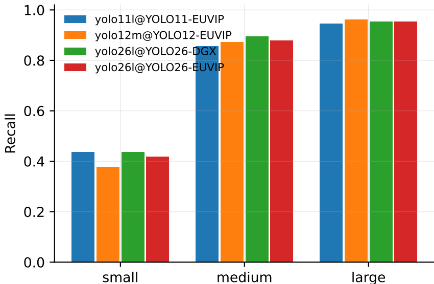
MDWD detection - recall by object size (test)
