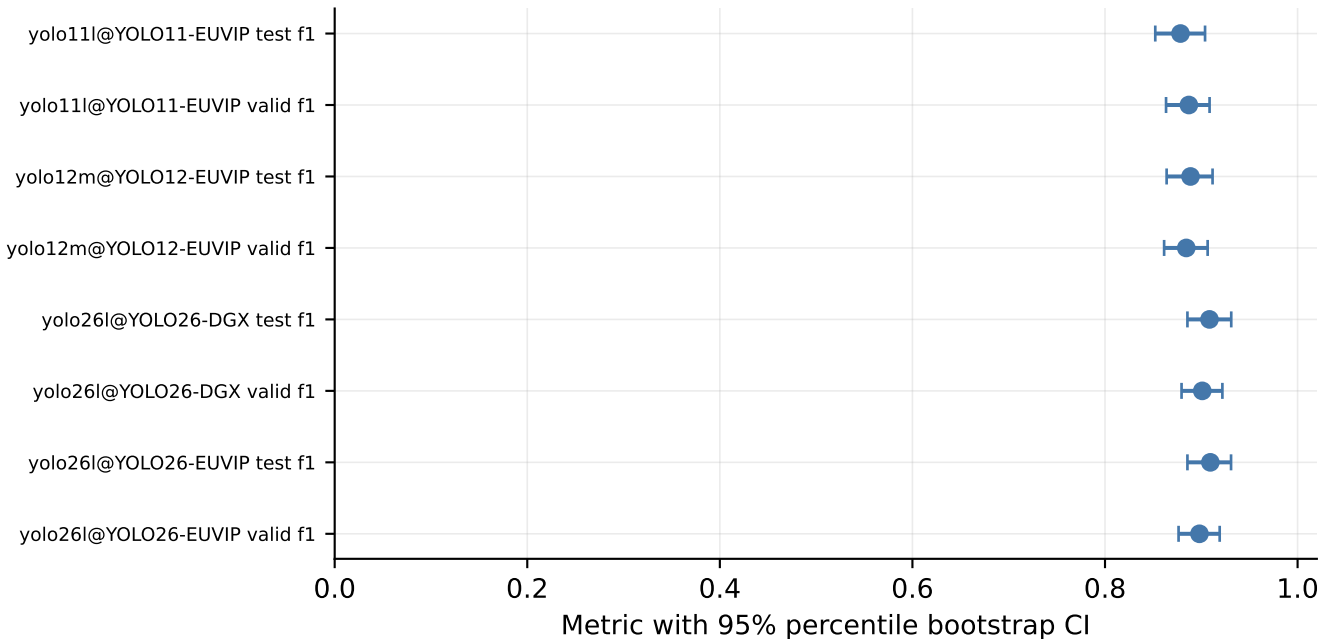
MDWD-detection - F1-family point estimates with CIs
