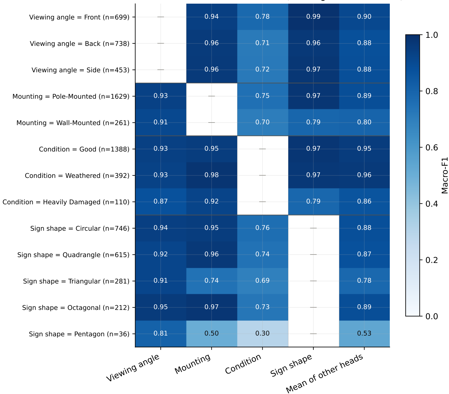
Cross-attribute semantic robustness (self-target slices omitted)
