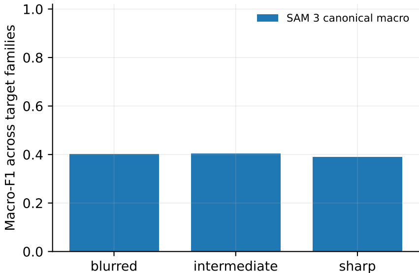
MTSD SAM 3 canonical - macro-F1 by sharpness
