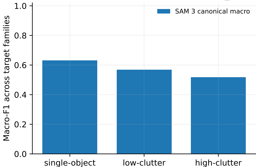
MDWD SAM 3 canonical - Macro-F1 by object_density
