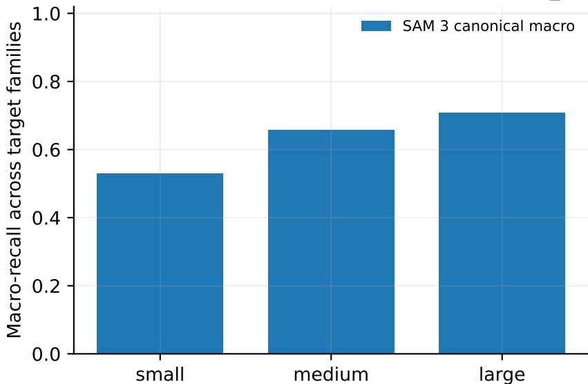
MDWD SAM 3 canonical - Macro-recall by object_size
