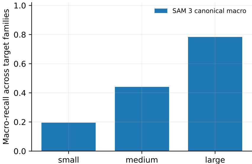
MTSD SAM 3 canonical - Macro-recall by object_size
