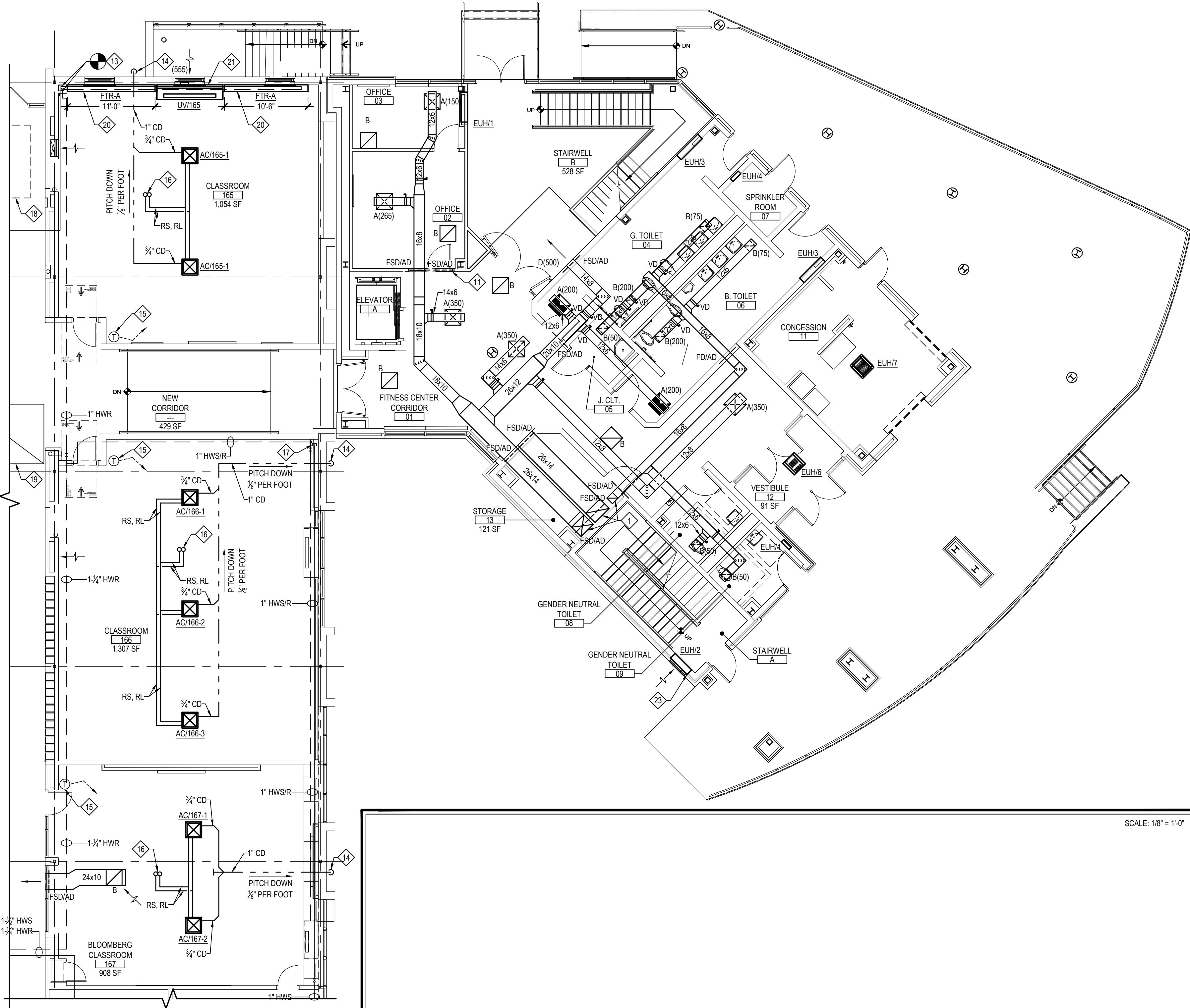
FIRST FLOOR MECHANICAL PLAN
