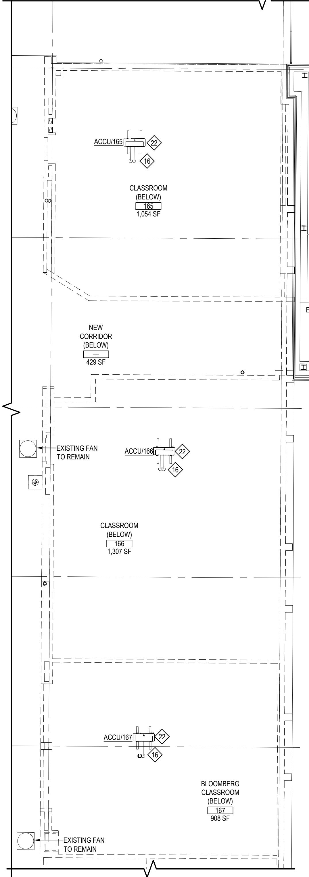
SECOND FLOOR MECHANICAL PLAN
