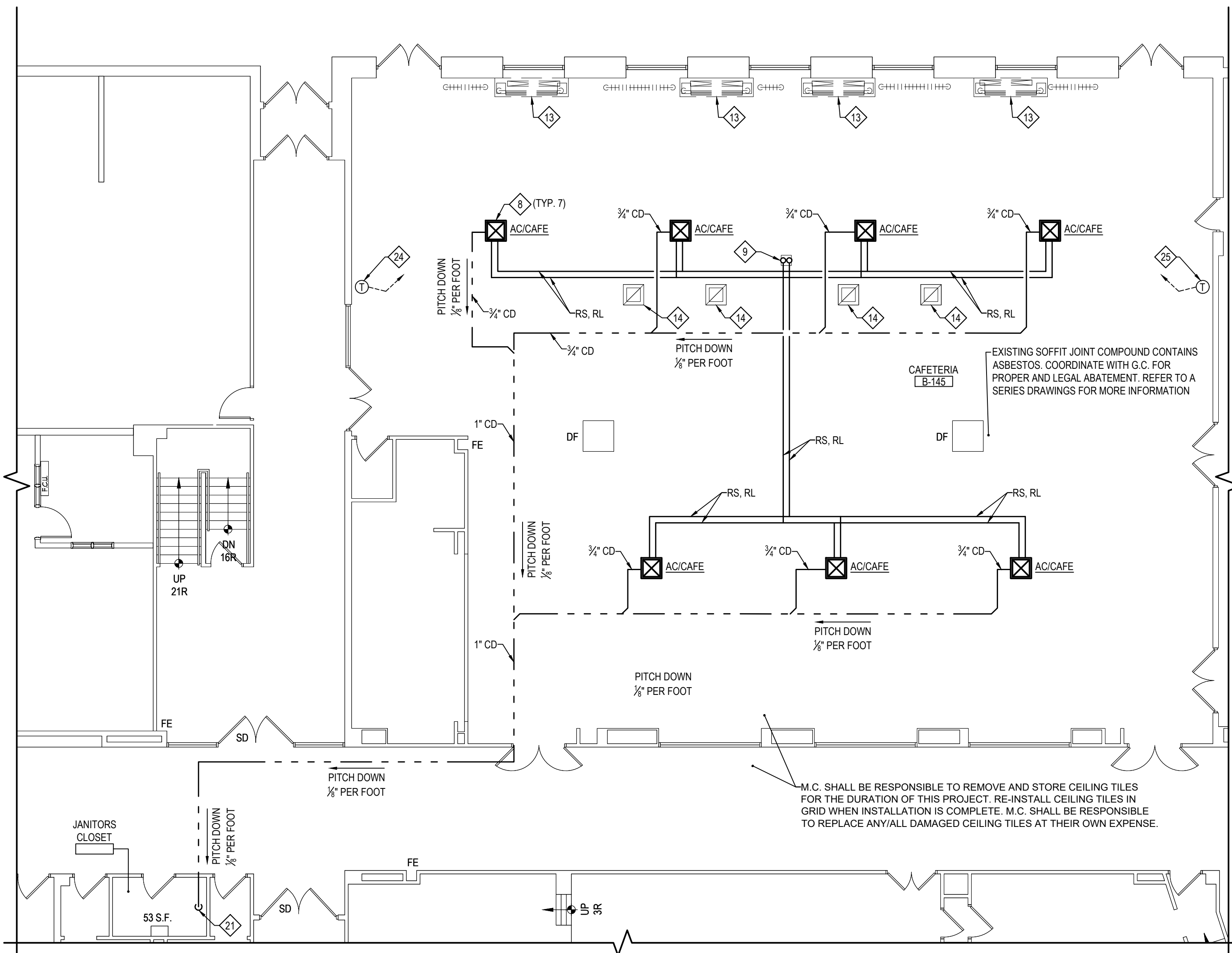
FIRST FLOOR CAFETERIA NEW WORK MECHANICAL PLAN
