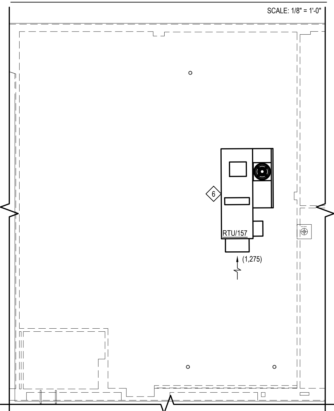
PARTIAL ROOF MECHANICAL NEW WORK PLAN - NEW ART ROOM 157
