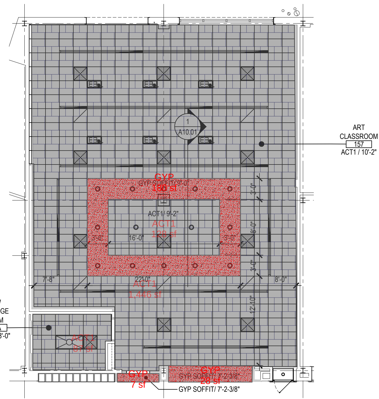
PARTIAL FIRST FLOOR REFLECTED CEILING PLAN - ART CLASSROOM 157
