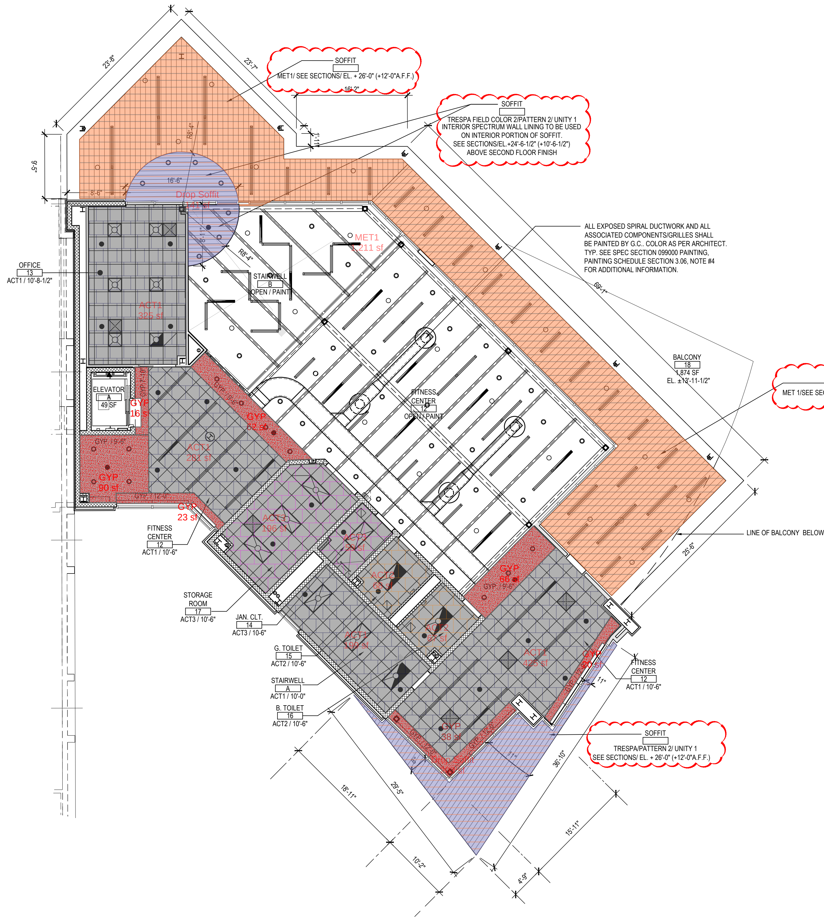
PARTIAL SECOND FLOOR REFLECTED CEILING PLAN - FITNESS CENTER
