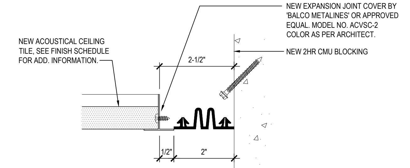
1 ACOUSTICAL CEILING TO WALL EXPANSION JOINT
