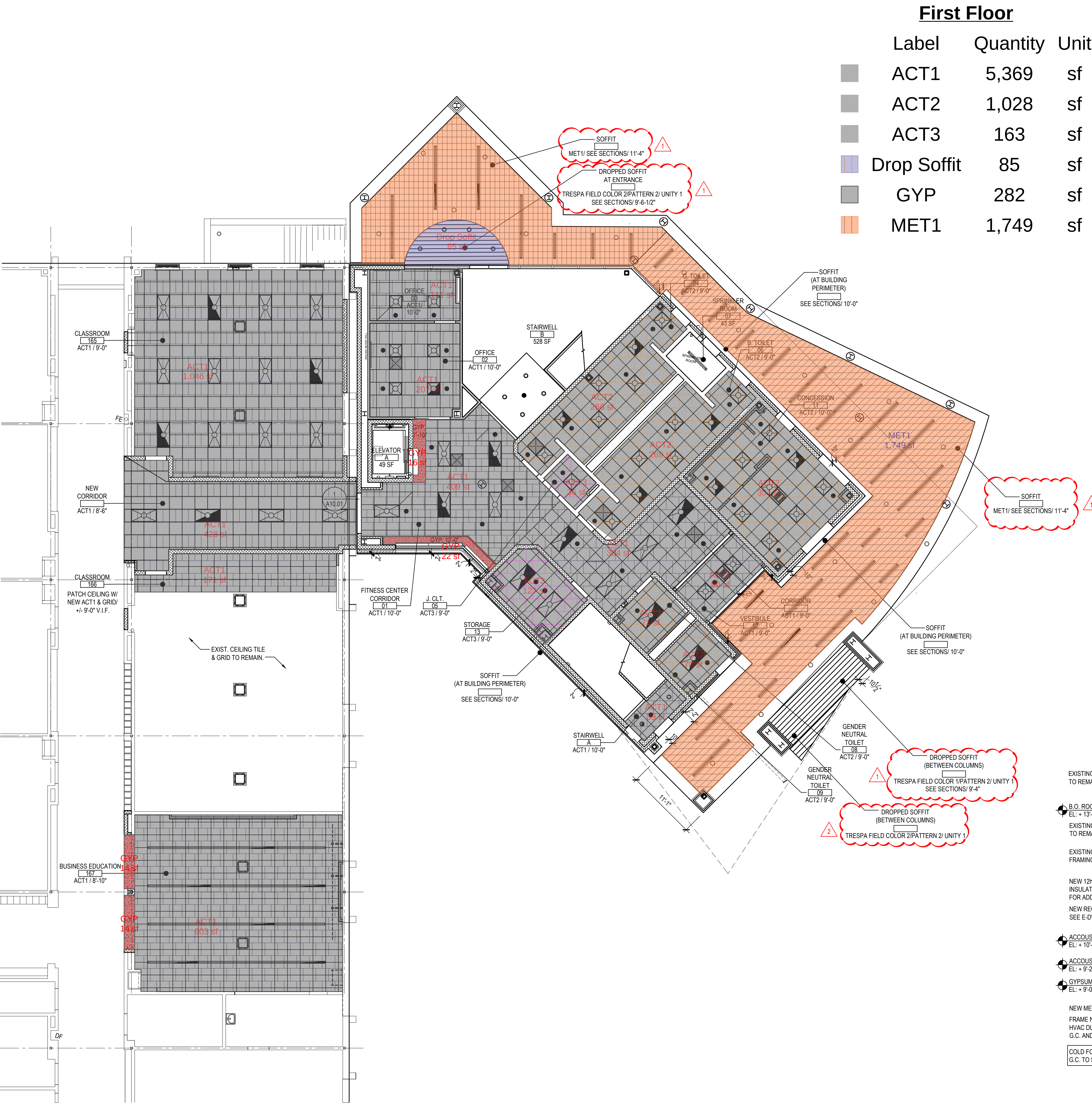
PARTIAL FIRST FLOOR REFLECTED CEILING PLAN - CLASSROOM 165, CLASSROOM 167, BUSINESS EDUCATION 167 & FITNESS CENTER
