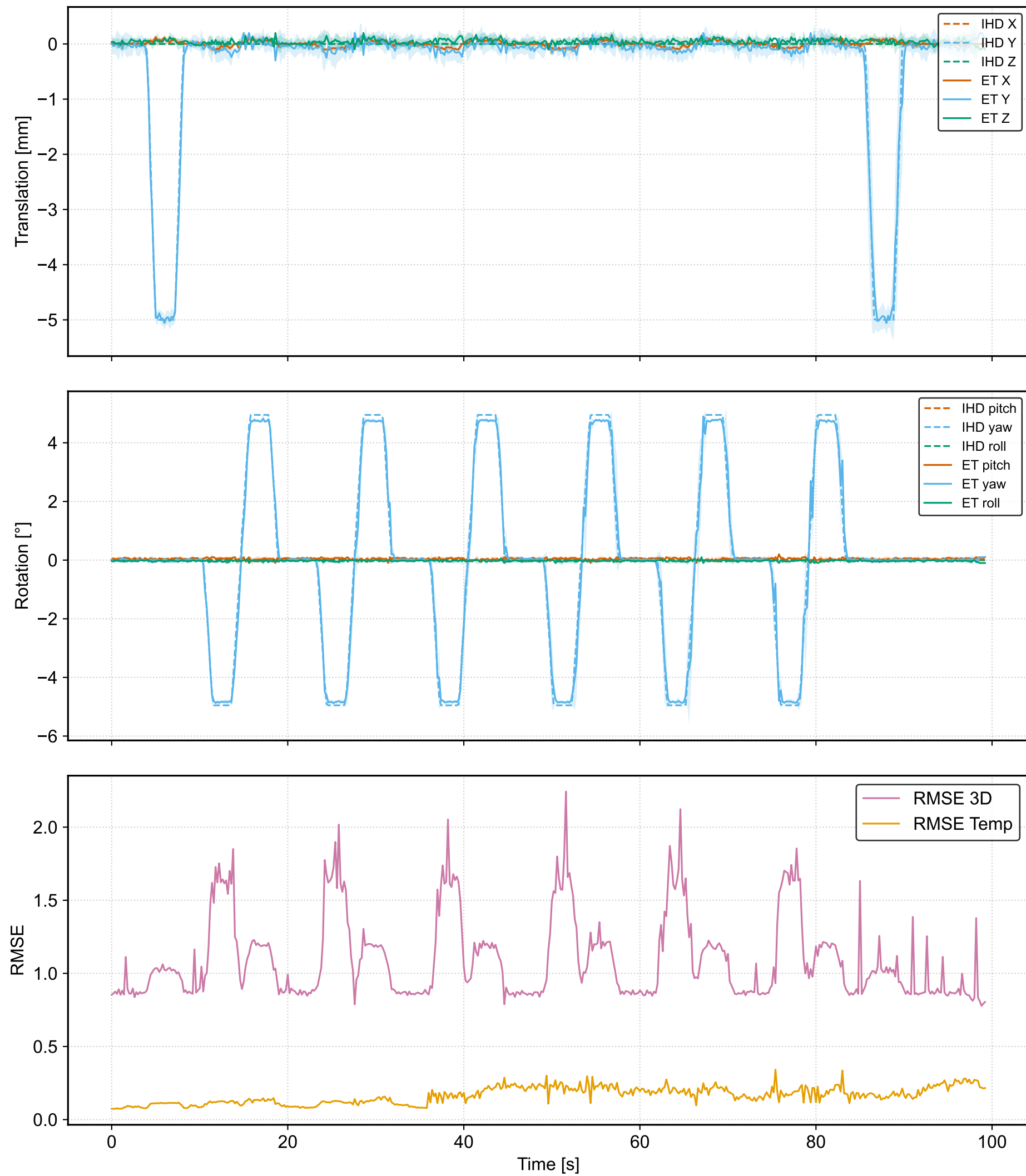
ExacTrac surface outputs vs. IHD (with moving axes: Rotation)
