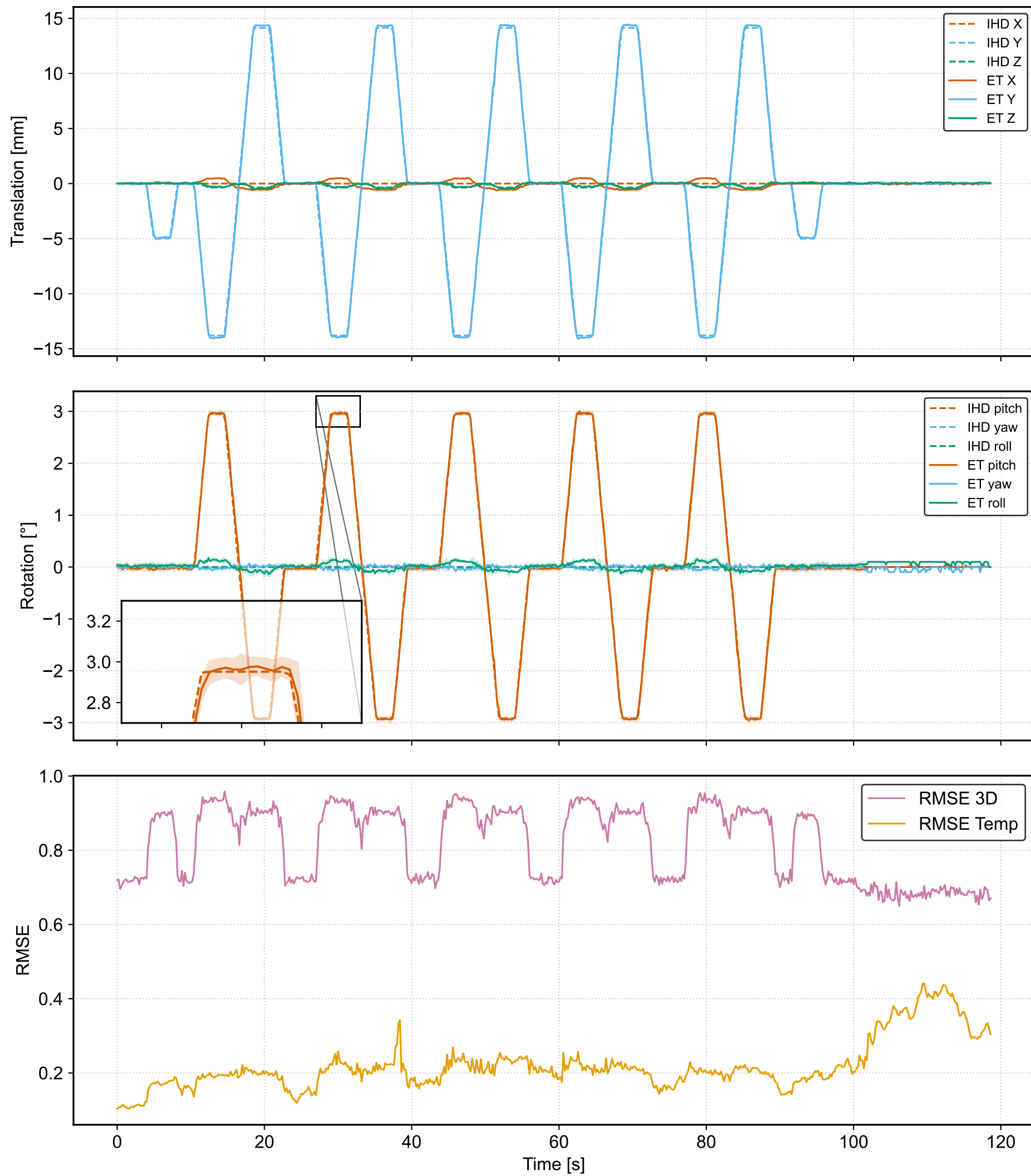
ExacTrac surface outputs vs. IHD (with moving axes: Vertical)
