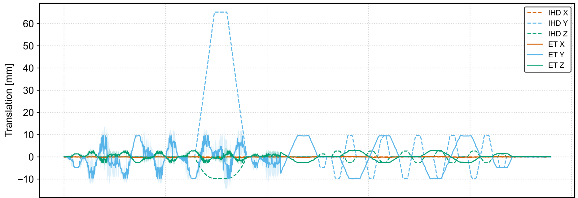
ExacTrac surface outputs vs. IHD (with moving axes: Vertical_Slide)
