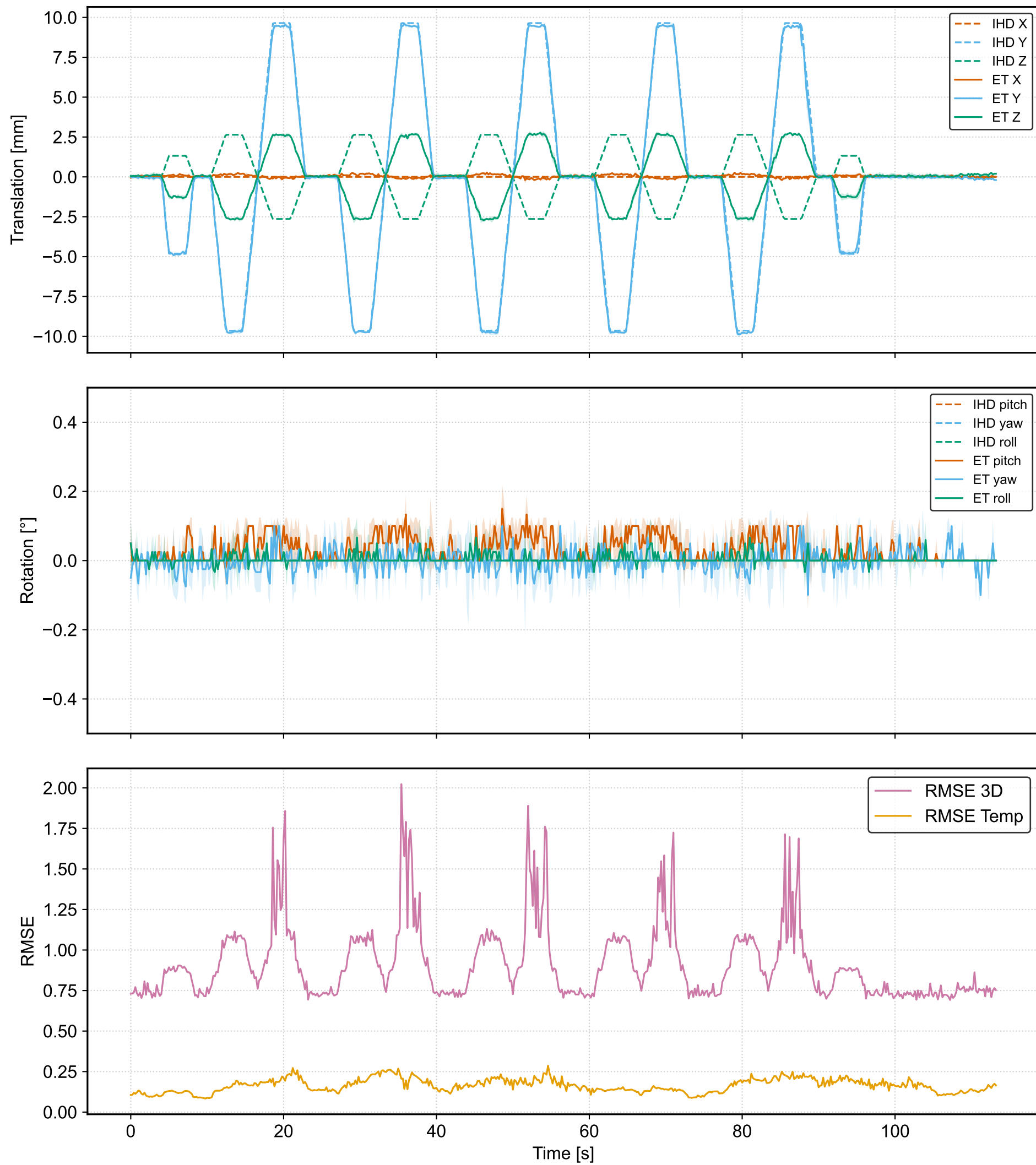
ExacTrac surface outputs vs. IHD(with moving axes: Vertical_Slide)
