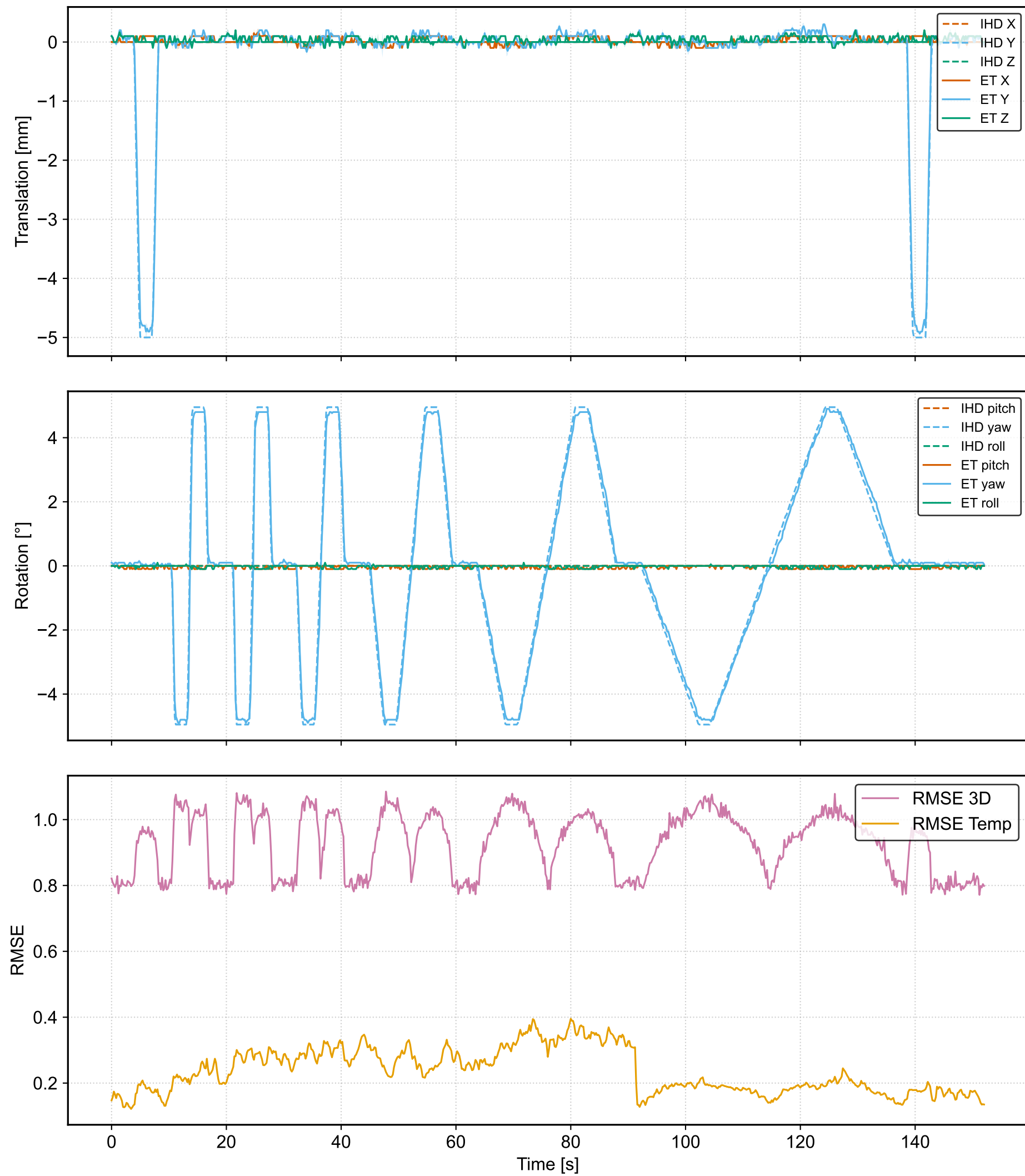
ExacTrac surface outputs vs. IHD (with moving axes: Variable_Geschwindigkeit)
