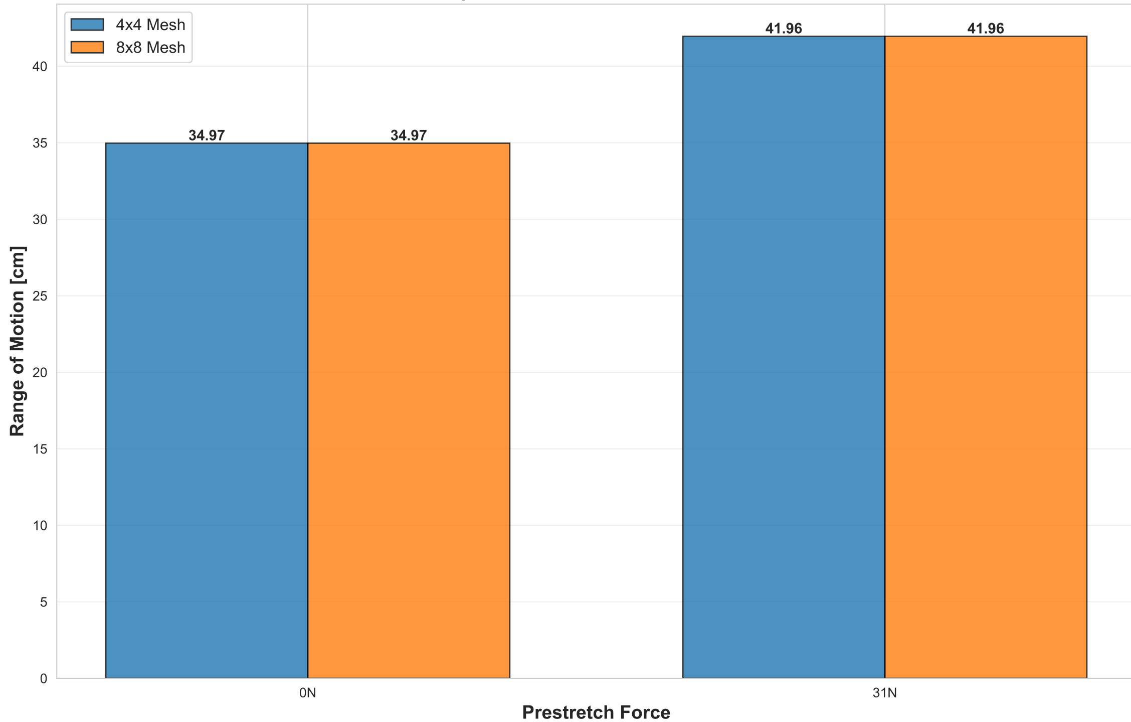
ROM Comparison: 4x4 vs 8x8 Mesh Resolution
