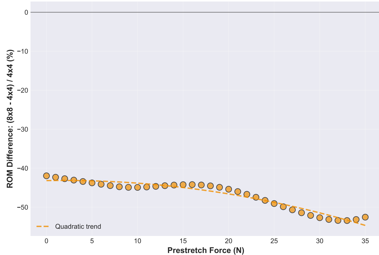
Mesh Resolution Effect on ROM (Relative Difference)
