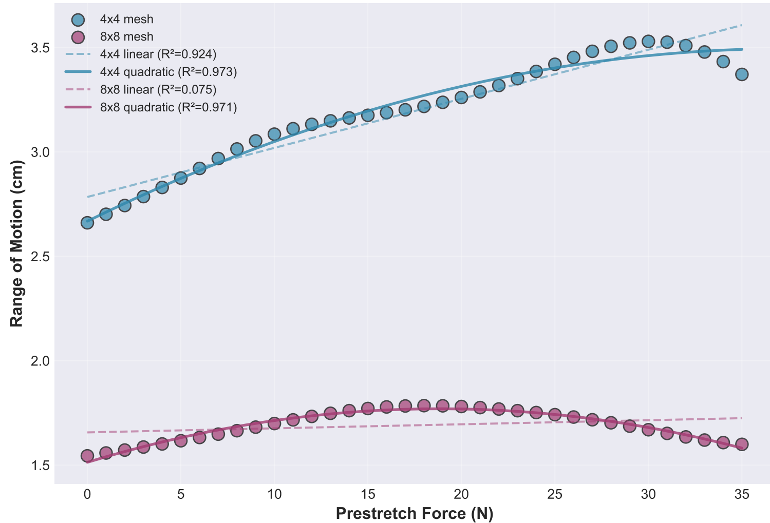
Force-ROM Relationship (Linear vs Quadratic Models)
