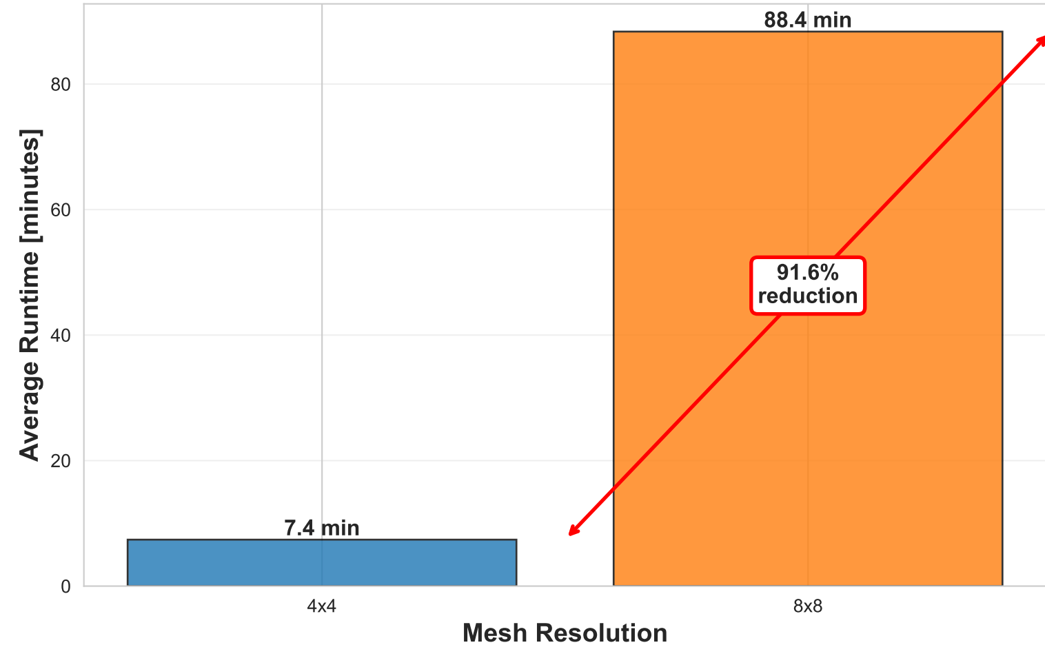
Average Runtime Comparison (Reduction: 91.6%)
