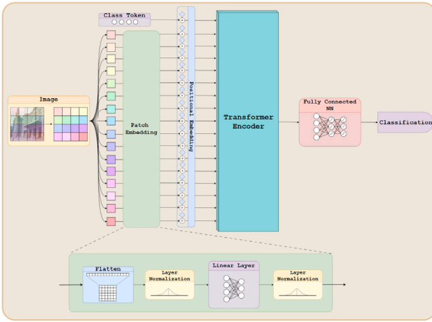
Fig. 4. ViT diagram of token projections.
