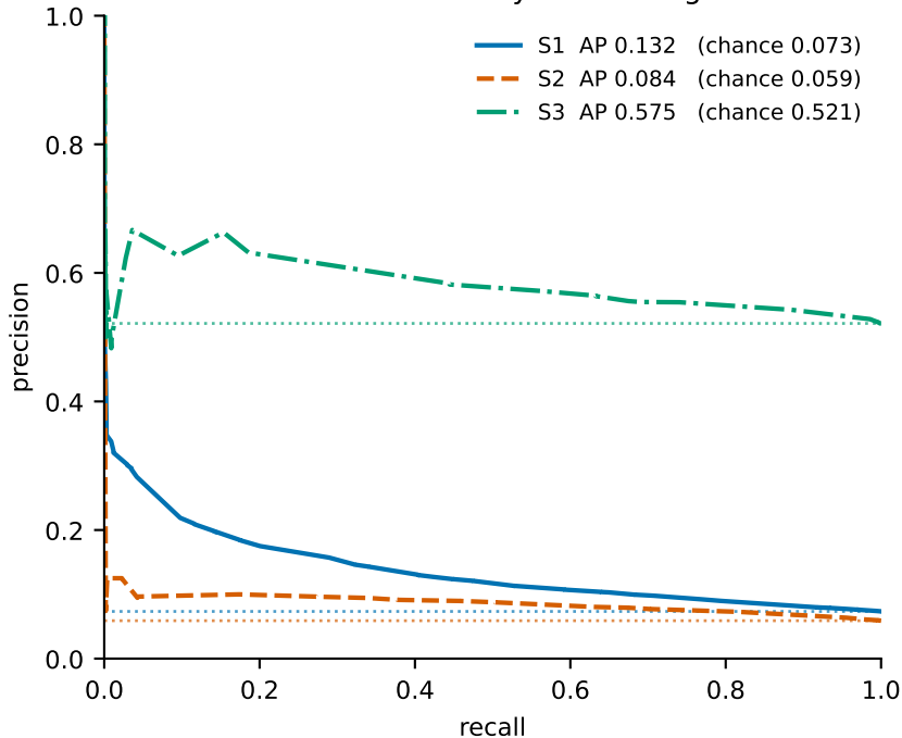
Precision-recall by funnel stage
