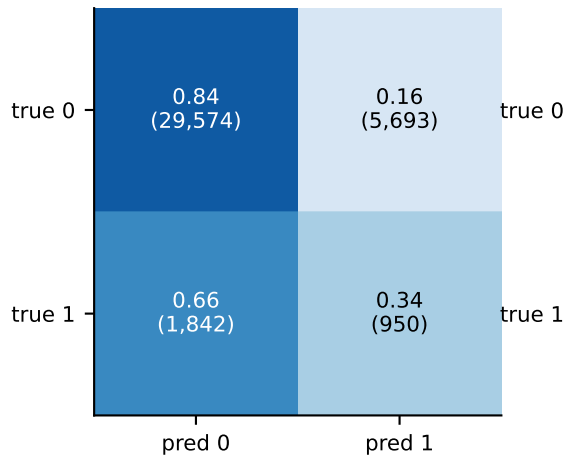
S1 (threshold 0.116)
