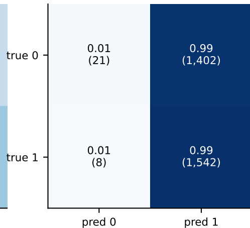
S3 (threshold 0.433)
