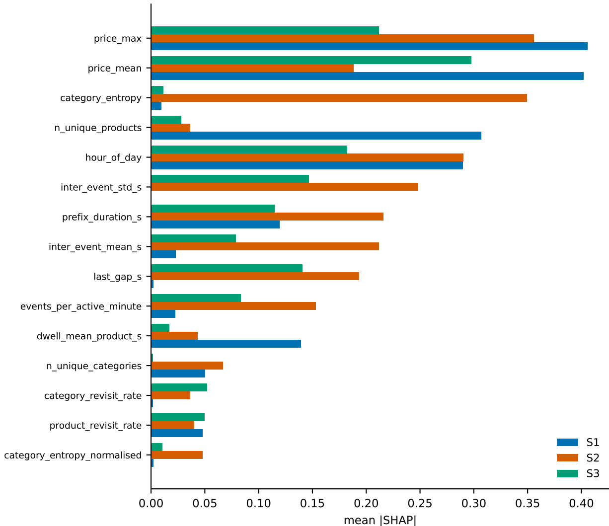
Ungrouped feature importance by stage (seed 42)
