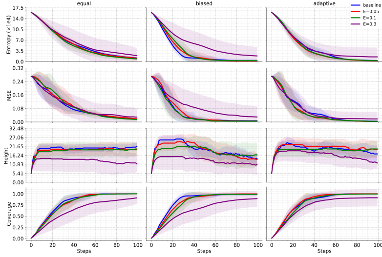
Fig. 2. Performance metrics are shown for the theoretical sensor model (baseline) and sampled models ( E = 0.05, 0.1, 0.3 ) for a Gaussian field with equal, biased, adaptive weights (presented left to right). Shaded areas represent standard deviation, and solid lines indicate mean values of 20 independent runs.
