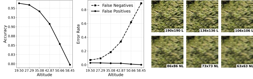
Fig. 4. Left/Center: Classification accuracy and FP, FN rates as functions of altitude, showing the trade-off between footprint size and image resolution. Gaussian blur simulates the image quality degradation at higher altitudes. Right: Example tile (47, 55) shown at varying altitudes, illustrating the effect of resolution on classification. For each altitude, corresponding crop size in pixels and the predicted class label (L – lodged, NL – not lodged) are indicated.
