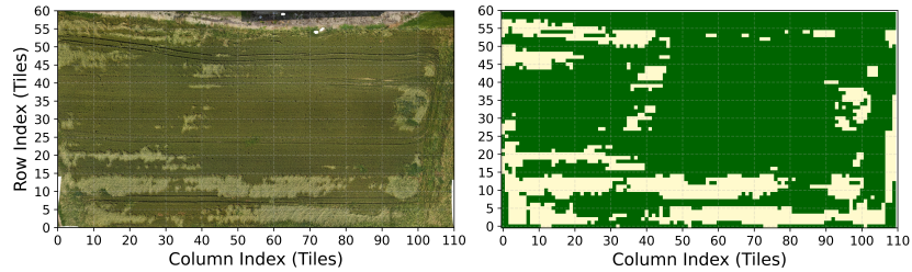
Fig. 3. Left: Orthomosaic of the wheat field divided into 1\text{ m} \times 1\text{ m} cells. Right: Manual annotation in the classes lodged (light yellow) and not lodged (dark green).
