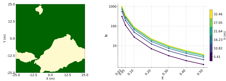
Fig. 1. Left: Gaussian random field generated with r = 4 , simulating a wheat field with lodging. Right: Required sample sizes computed from the theoretical sensor model ( a = 1 , b = 0.015 ) across different altitudes and precision levels.
