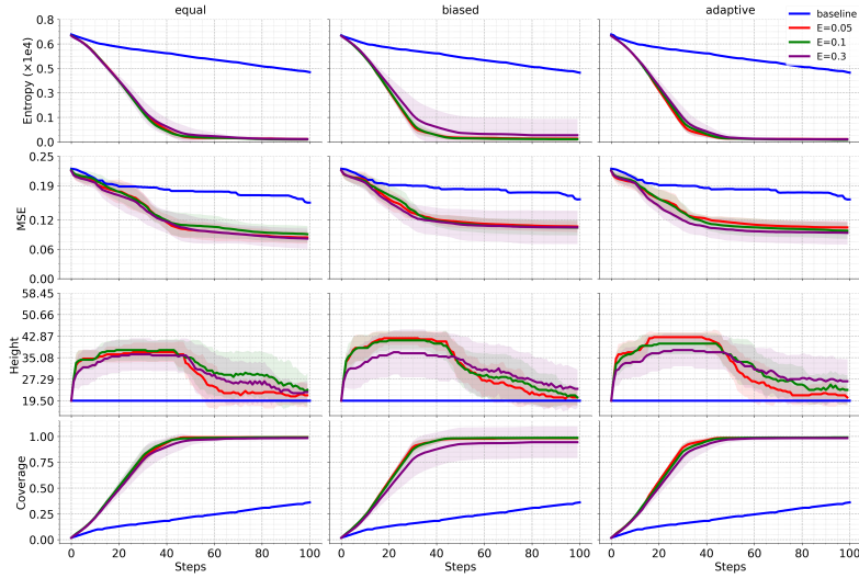
Fig. 5. Performance metrics are shown for the lawnmower strategy (baseline) and sampled models ( E = 0.05, 0.1, 0.3 ) for a orthomap field and pairwise equal, biased, and adaptive weights. Shaded areas represent standard deviation, and solid lines indicate mean values.
