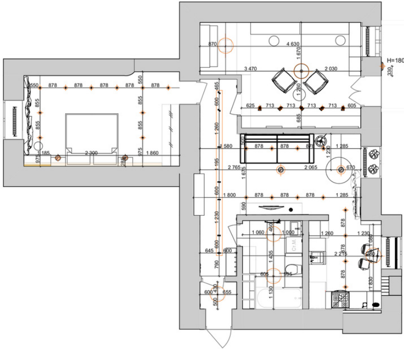
Lighting plan with furniture
