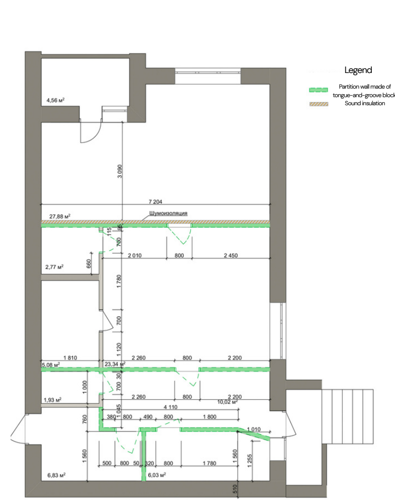
Installation plan 1:100
