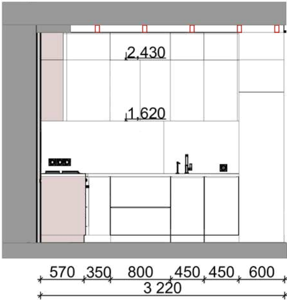
Kitchen sections
