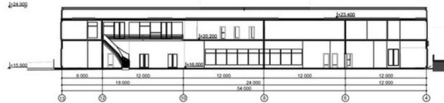
Section 1-1 1:500
