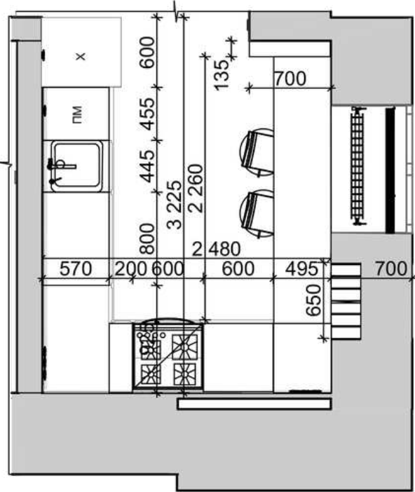
Kitchen plan 1:50
