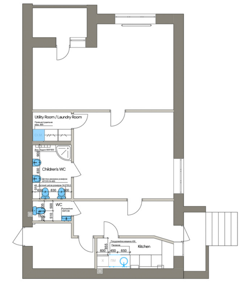
Plumbing plan 1:100
