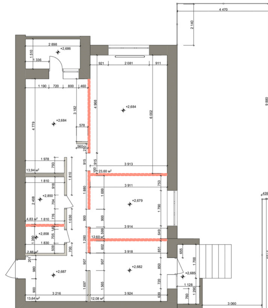
Demolition plan 1:100
