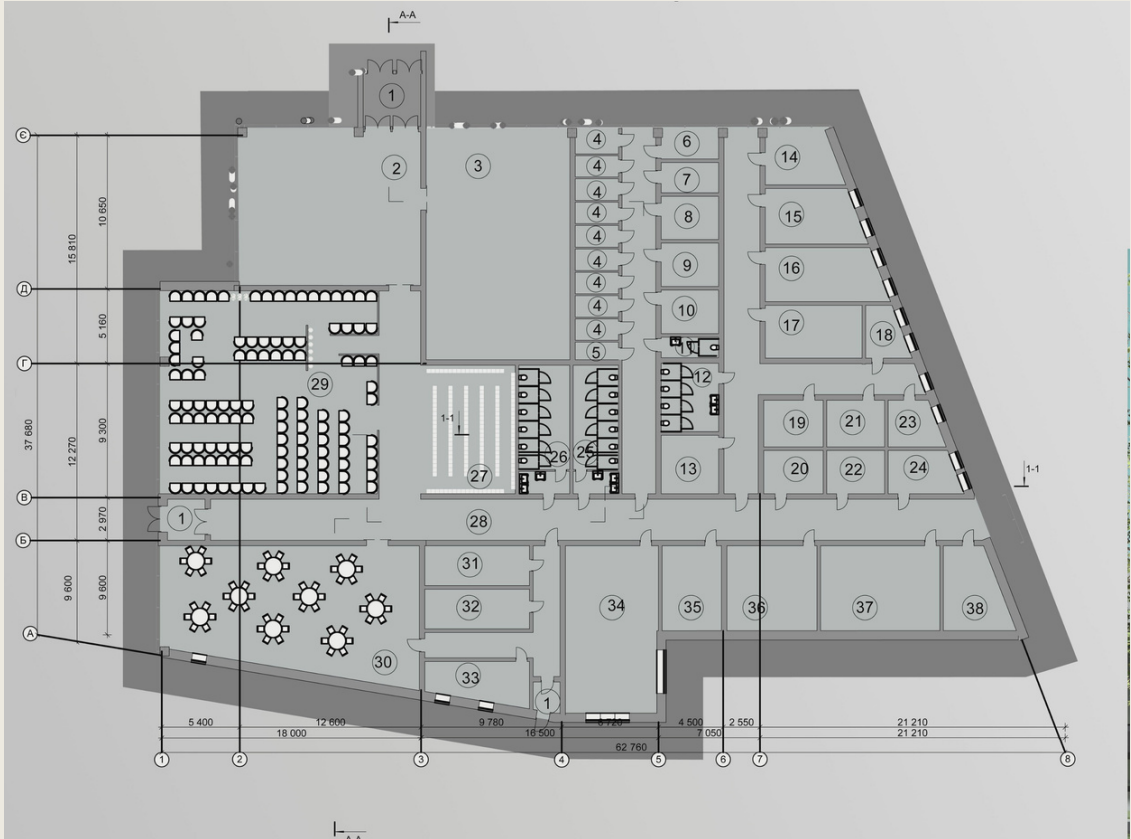
A bus terminal for 400 passengers includes a forecourt, a public transport stop nearby, a parking area, a boarding platform, a retail zone, and designated spaces for bus layover and maintenance.
