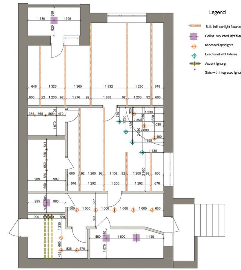
Lighting plan 1:100
