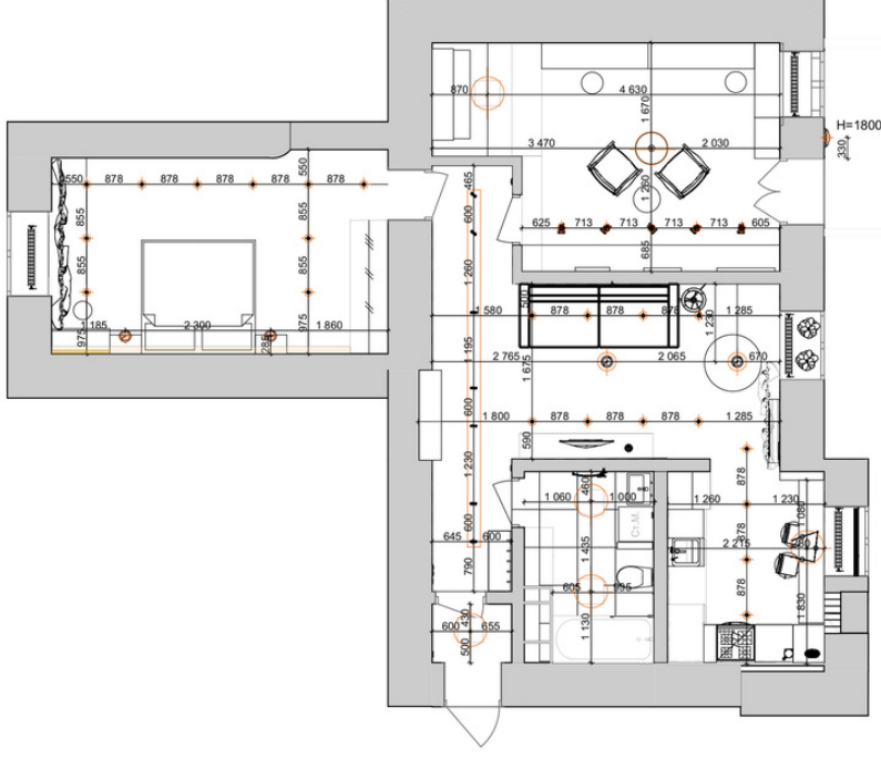
Lighting plan with furniture
