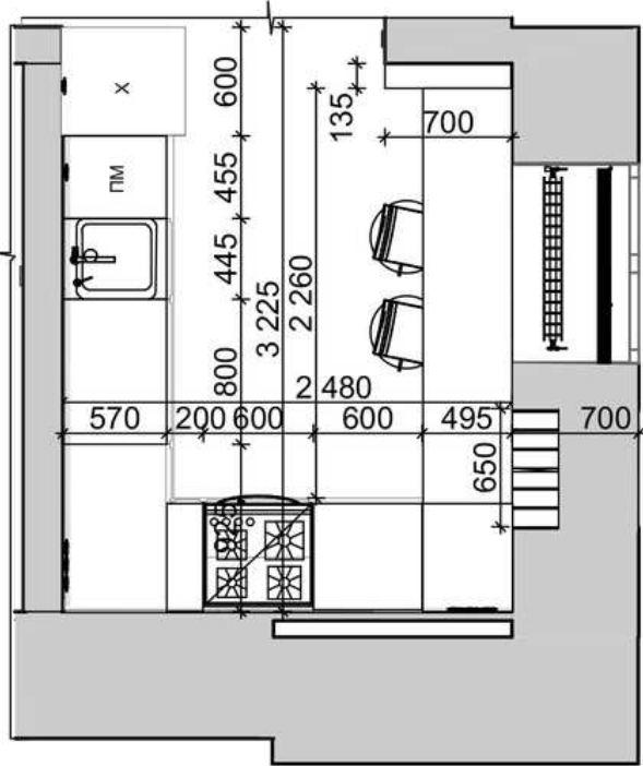
Kitchen plan 1:50
