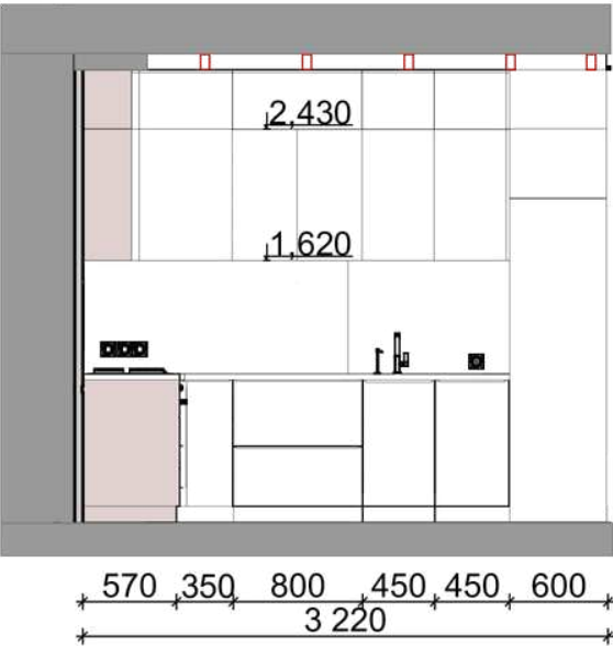
Kitchen sections
