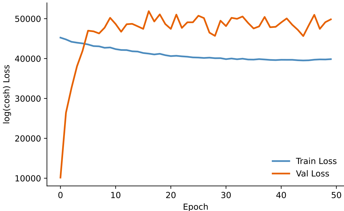
GNN Convergence Curve
