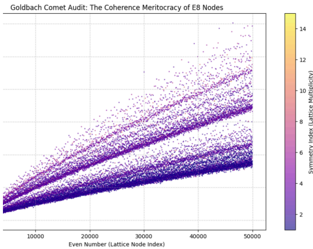
Fig. 38.3 The Goldbach comet, showing stratified bands of prime-pair abundance across even-number nodes.
