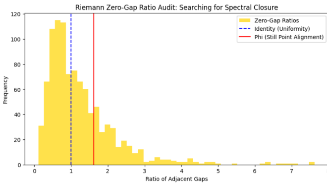
Fig. 38.2 Riemann zero-gap ratio audit with the identity line and the \phi alignment marker.
