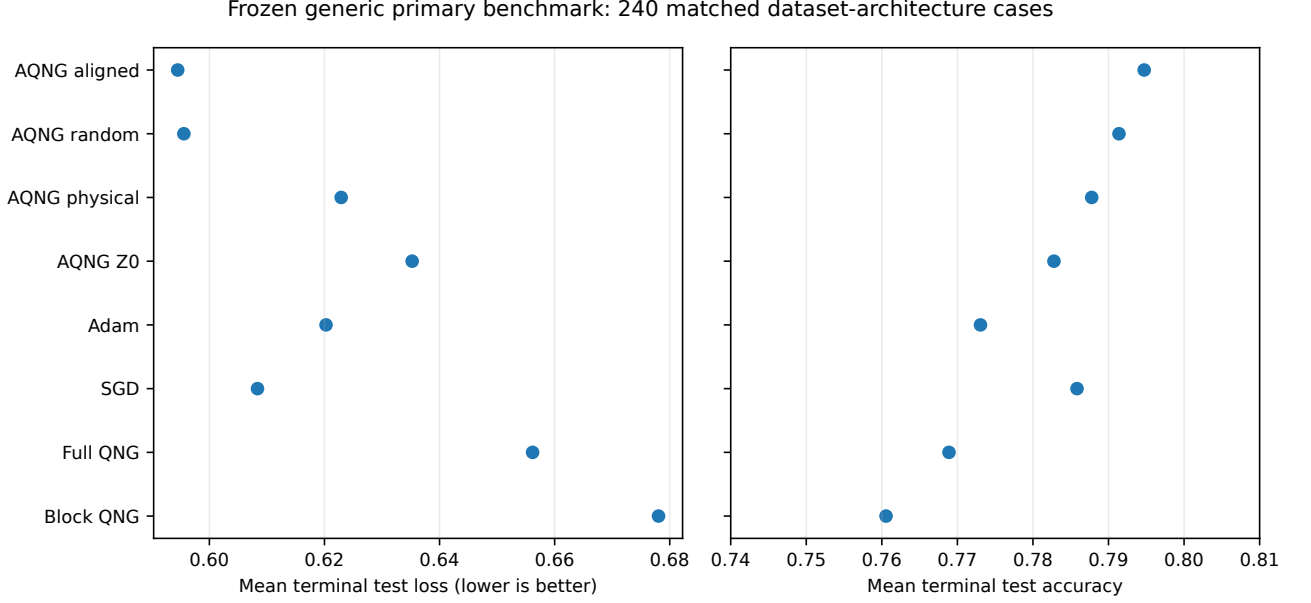
FIG. 2. Frozen generic primary benchmark pooled over the 240 nonconserving dataset–architecture cases. The primary protocol compares eight methods at matched data partitions and stochastic seeds. Aligned AQNG has the lowest pooled mean terminal test loss (0.5945) and highest pooled mean accuracy (0.7947), but random AQNG and SGD remain close. The pooled means are descriptive summaries; inferential claims use paired tests rather than treating all terminal rows as independent replicates.
