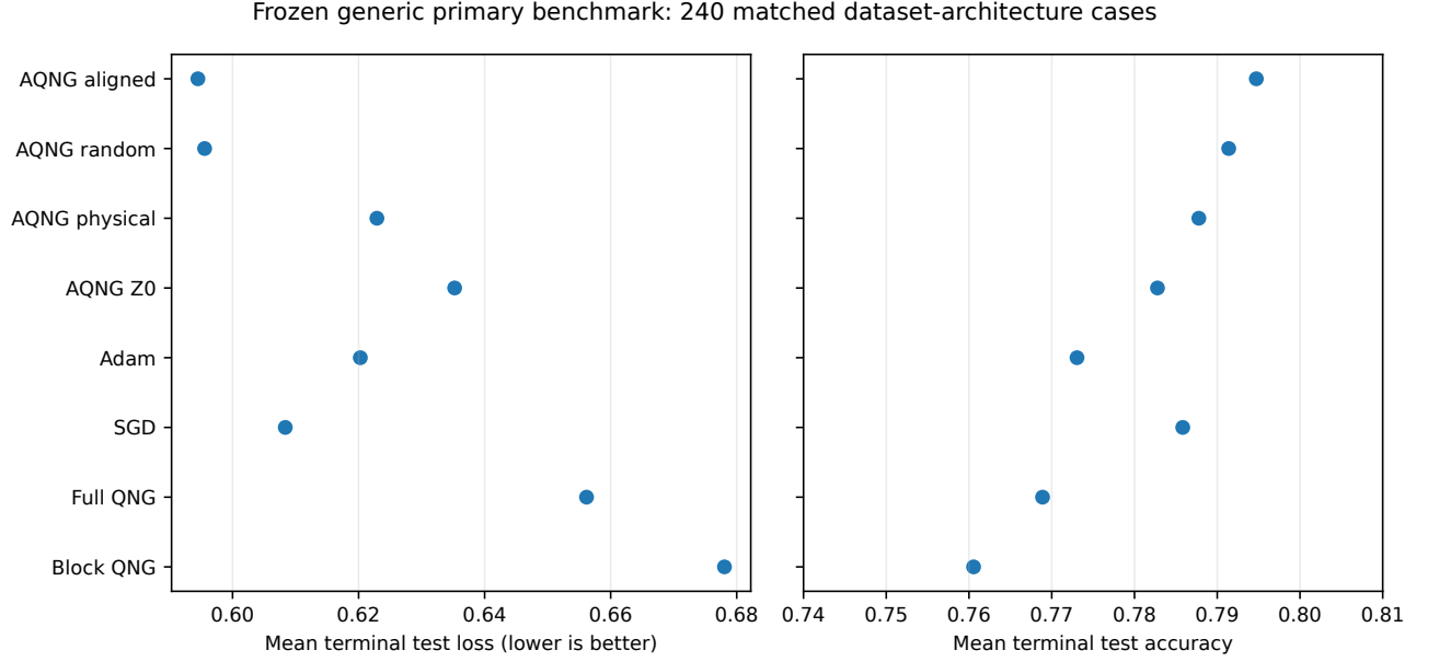
FIG. 7. Frozen generic primary benchmark pooled over the 240 nonconserving dataset–architecture cases. The primary protocol compares eight methods at matched data partitions and stochastic seeds. Aligned AQNG has the lowest pooled mean terminal test loss (0.5945) and highest pooled mean accuracy (0.7947), but random AQNG and SGD remain close. The pooled means are descriptive summaries; inferential claims use paired tests rather than treating all terminal rows as independent replicates.
