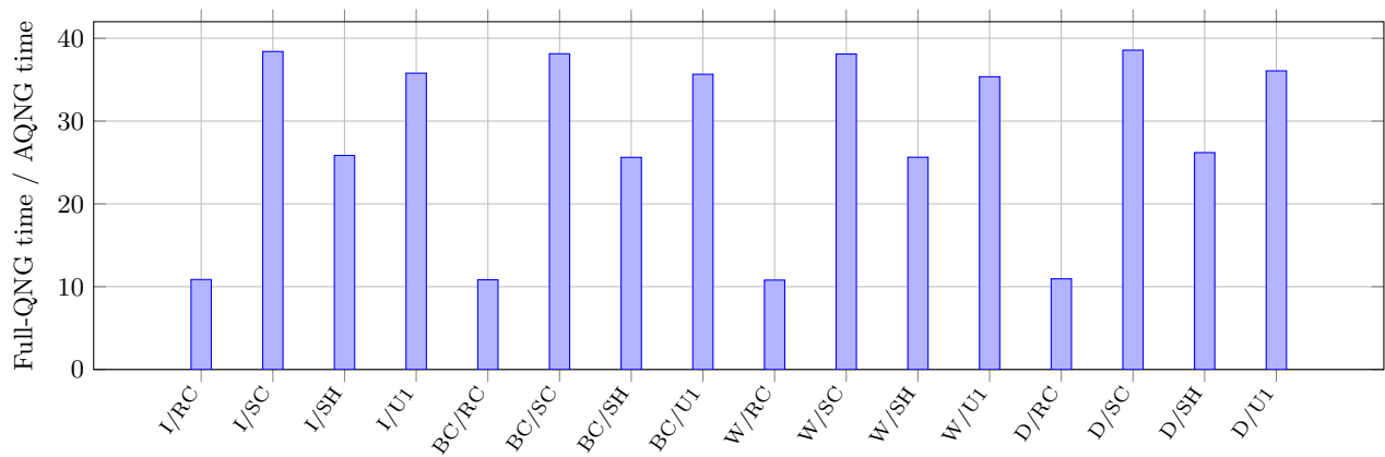
FIG. 4. Backend-specific mean wall-clock ratio, Full QNG divided by AQNG. The ratio is approximately 11\times for RyRz-CZ, 38\times for SU(2)-CNOT, 26\times for SU(2)-Haar, and 35\text{--}36\times for U(1). Because the metric paths use different simulator backends, this figure is an implementation benchmark rather than an intrinsic complexity claim.
