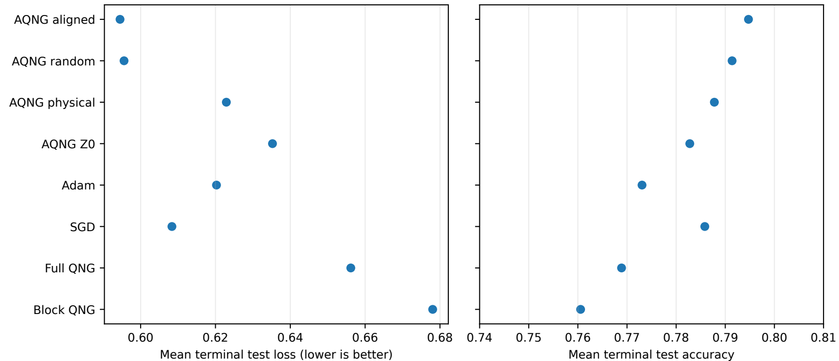
Frozen generic primary benchmark: 240 matched dataset-architecture cases
