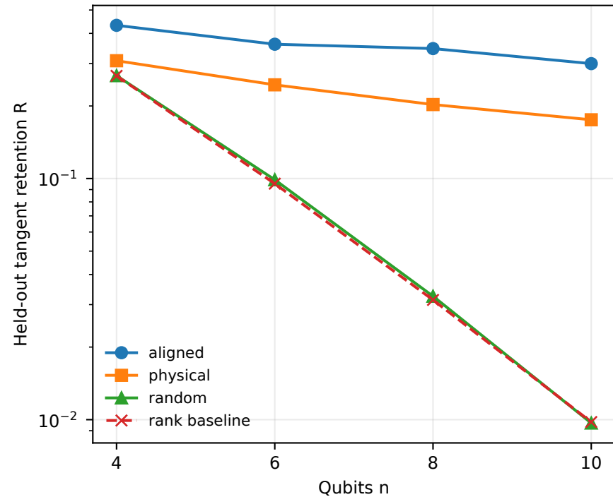
SU(2)-Haar: rank law remains clean while orientation gain grows
