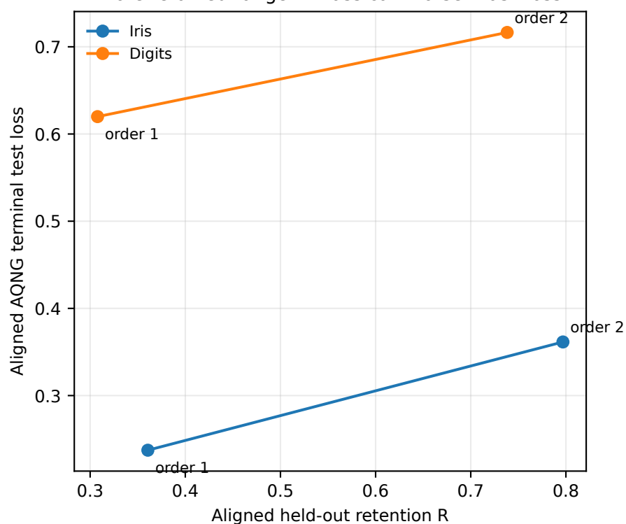
More retained tangent mass can worsen task loss
