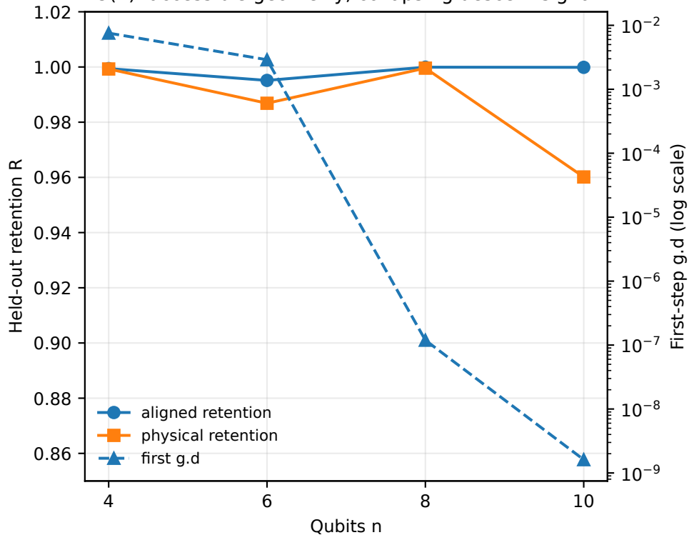
U(1): accessible geometry, collapsing descent signal
