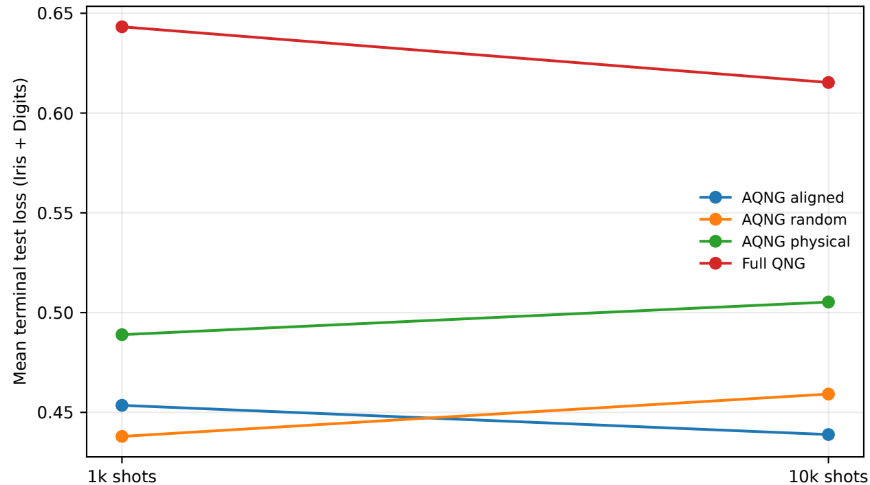
Finite-shot SU(2)-Haar robustness Full QNG uses an analytic metric oracle in this protocol
