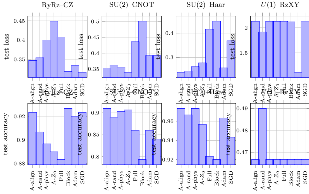
FIG. 6. Iris primary benchmark. Top row: mean terminal test loss. Bottom row: mean terminal test accuracy. Columns correspond to the four circuit families.
