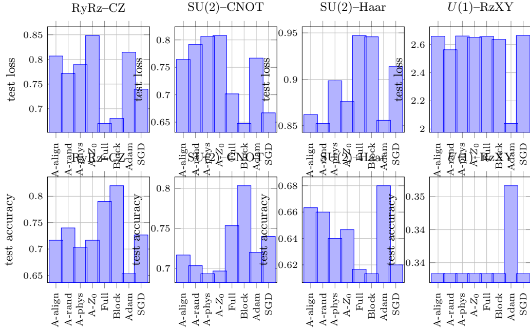
FIG. 7. Breast Cancer primary benchmark. Top row: mean terminal test loss. Bottom row: mean terminal test accuracy. Columns correspond to the four circuit families.
