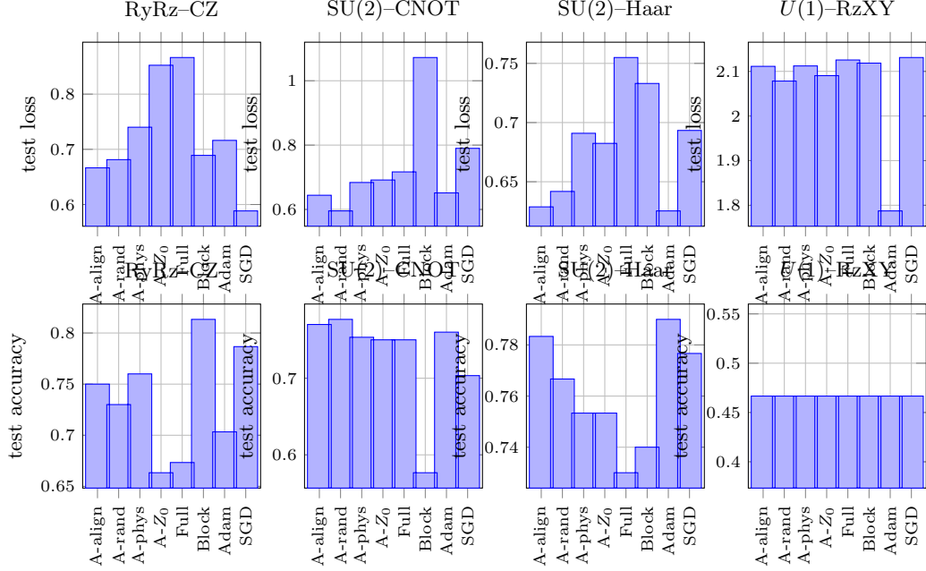
FIG. 9. Digits primary benchmark. Top row: mean terminal test loss. Bottom row: mean terminal test accuracy. Columns correspond to the four circuit families.
