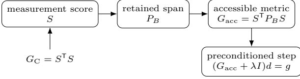
FIG. 1. Accessible natural-gradient construction. The retained readout span projects the measurement score before the pullback metric is formed; the resulting metric preconditions the task gradient.
