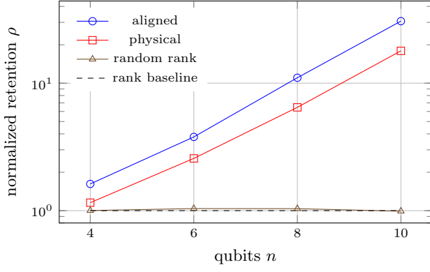
FIG. 2. SU(2)-Haar qubit scaling. The random rank-matched control remains close to \rho = 1 , whereas the structured readouts become increasingly super-baseline with system size.
