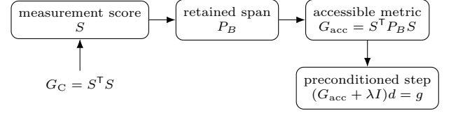
FIG. 1. Accessible natural-gradient construction. The retained readout span projects the measurement score before the pullback metric is formed; the resulting metric preconditions the task gradient.
