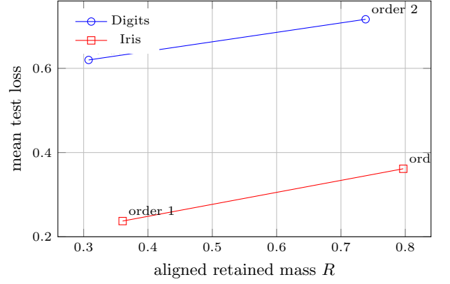
FIG. 3. Readout-order tradeoff for aligned AQNG on SU(2)-Haar. Moving from weight-one to weight-two diagonal readouts increases retained tangent mass but also increases mean test loss on both datasets.
