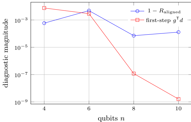
FIG. 4. Diagnostic separation in the number-conserving U(1) scaling control. The aligned readout remains nearly complete, while the first-step descent signal collapses by several orders of magnitude.
