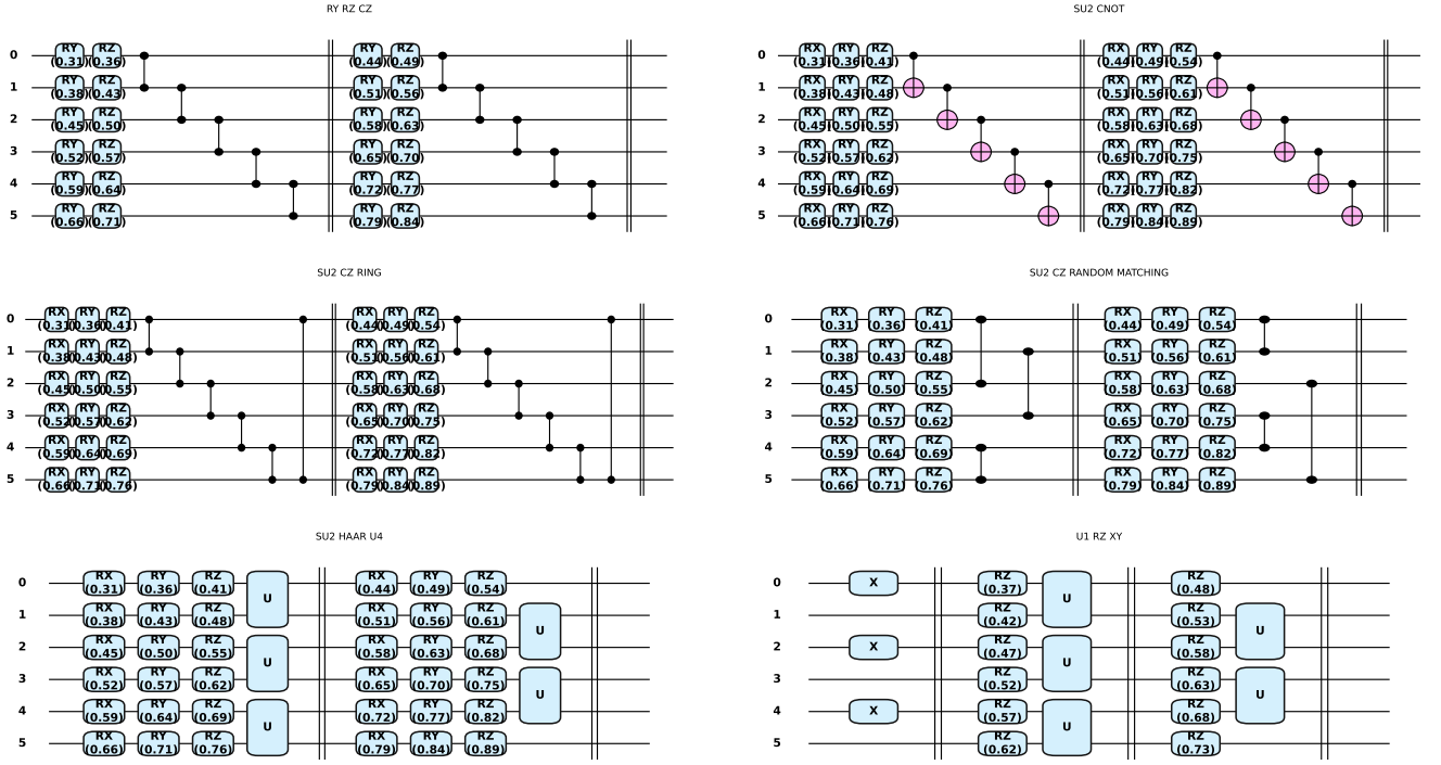
FIG. 3. Circuit families used in the numerical campaign, rendered directly from PennyLane circuit definitions [35]. From top left to bottom right: RY-RZ-CZ line, SU2-CNOT line, SU2-CZ ring, SU2-CZ random matching, SU2-Haar- U(4) brickwork, and the half-filled U(1) RZ-XY line. For legibility the drawings show n = 6 and two representative layers; the production simulations use the depths and system sizes specified in the numerical protocol. The U(1) panel begins from the alternating half-filled computational-basis state, matching the simulation code. Generic unitary boxes in the last row represent the actual two-qubit matrices used by the simulator rather than a gate decomposition.
