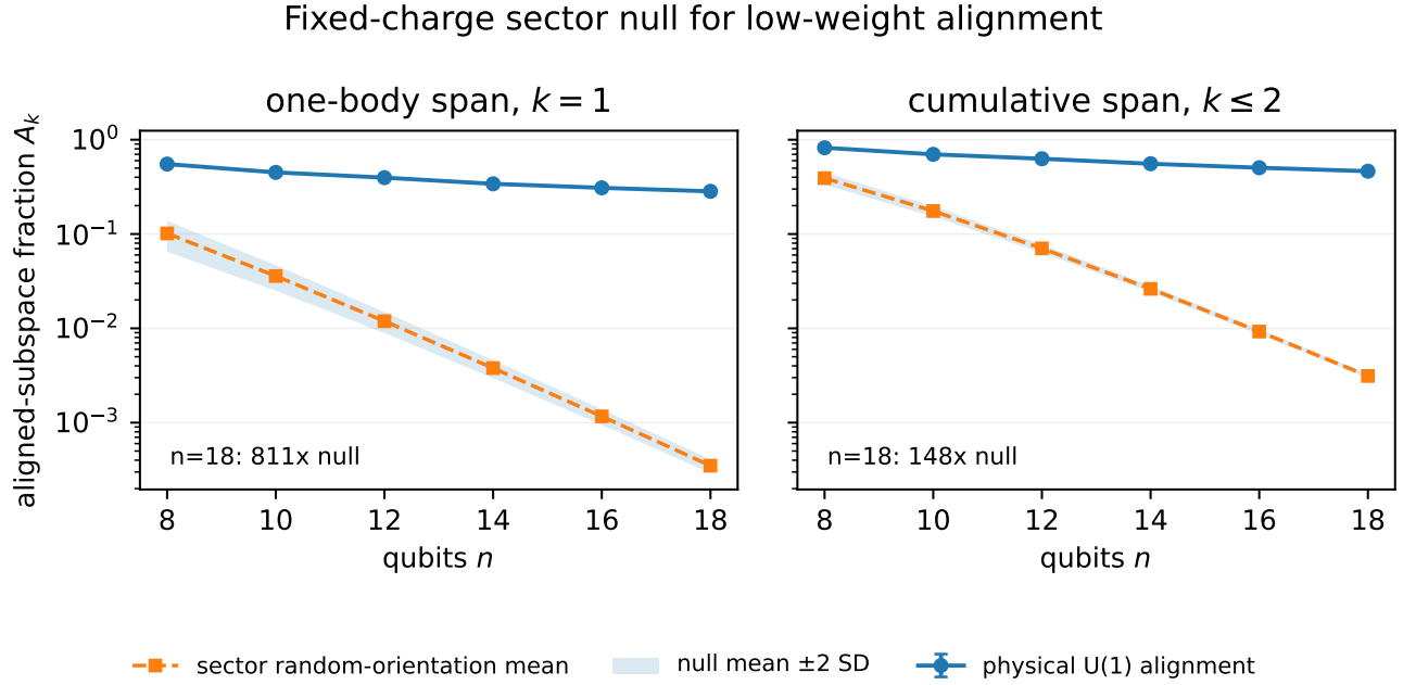
FIG. 6. Sector-corrected random-orientation control for the half-filled U(1) alignment statistic. The null draws the leading rank- r_1 subspace randomly inside the same half-filled centered score sector, rather than comparing with the full computational-basis score space. Points are the measured cross-fitted alignment means with circuit-bootstrap intervals; dashed curves are the exact random-orientation means and shaded bands show two null standard deviations from Grassmann projector moments. The observed alignment remains orders of magnitude above the sector null at the largest sizes.
