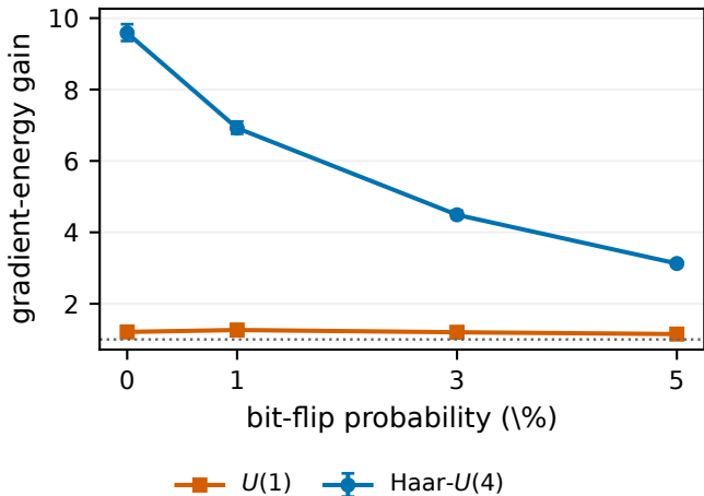
Readout-noise robustness
